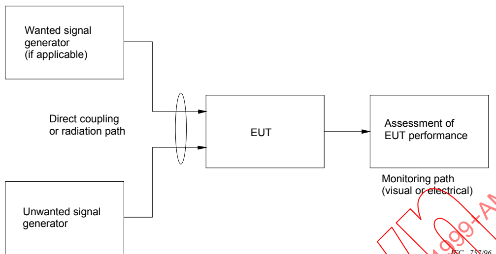
Figure 17 – Fundamental concept of immunity measurement (see 3.1.1)
