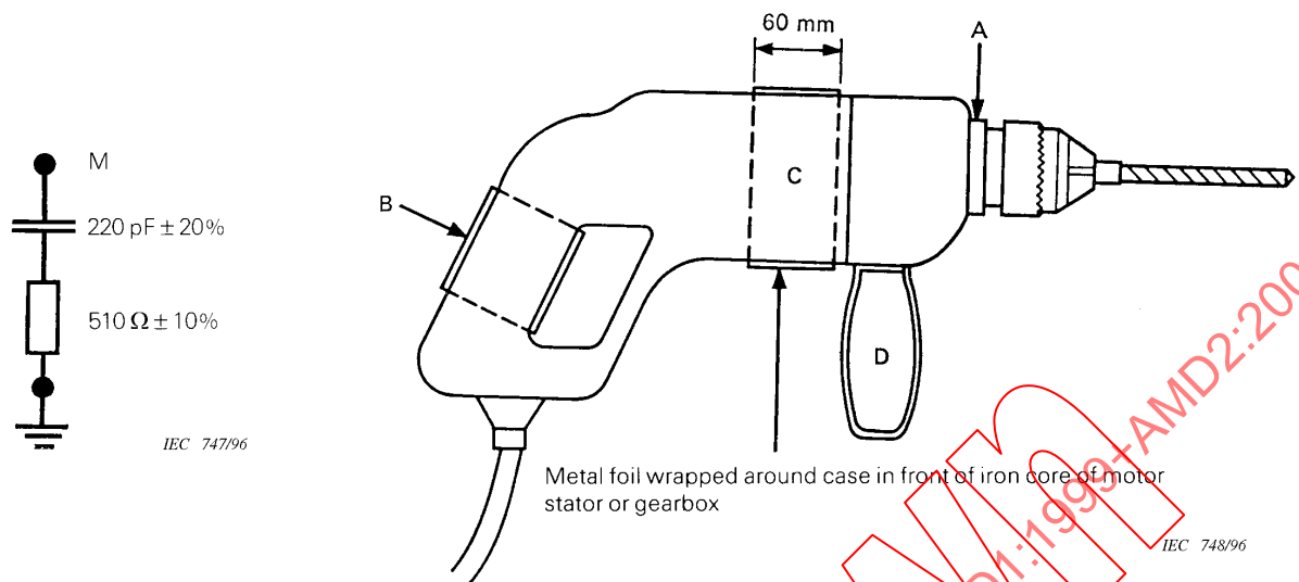
Figure 8 – RC element for artificial hand (see 2.4.4.2.3)
