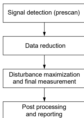
Figure 22 – Generic process to help reduce measurement time
