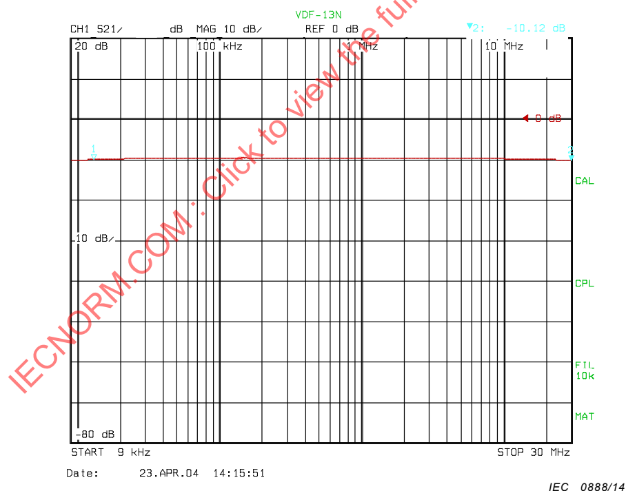
Figure E.3 – Impedance measured with the arrangement of Figure E.2 both with reference to the front panel ground and to the grounding sheet
