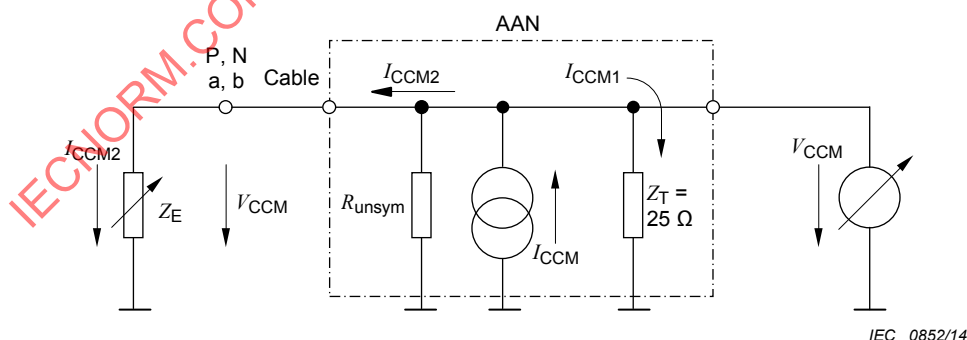
Figure 8 – Illustration of current I_{CCM}
