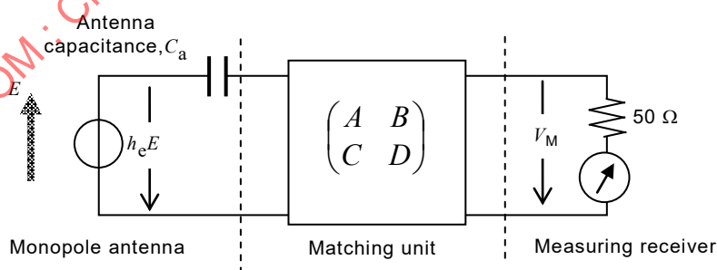
Figure G.6 – Equivalent circuit representation for a monopole antenna system
