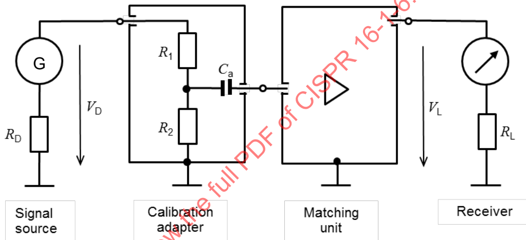
Figure G.10 – Circuit for dummy antenna simulating the effects of the antenna effective height, h_e
