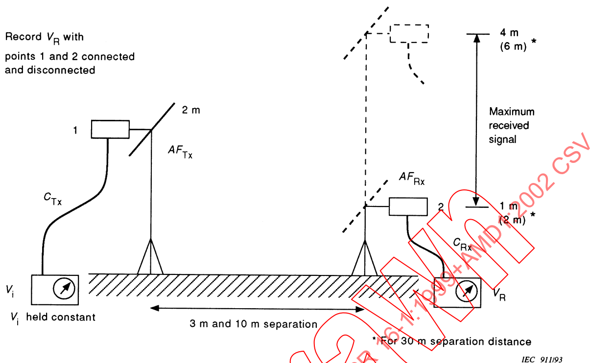
Figure 16 – Configuration of equipment for measuring horizontal polarization of site attenuation (see 5.6.6 and annex G)
