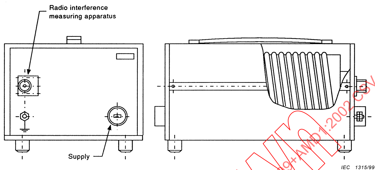
Figure 28 – A general view of the artificial mains network (see F.7.2)
