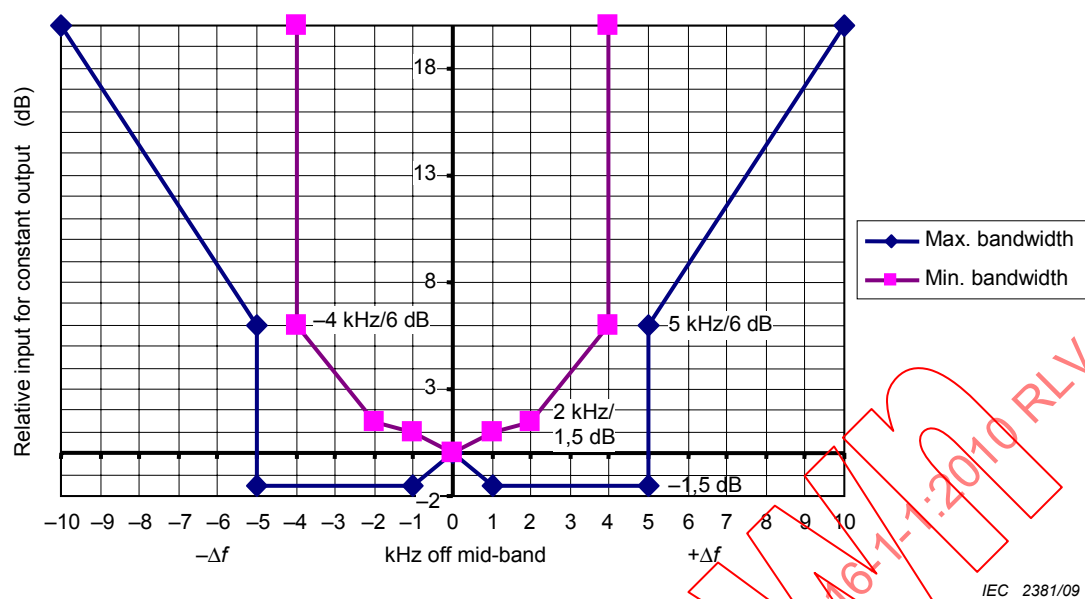
Figure 2b) – Limits of overall selectivity – Pass band (see 4.5.1, 6.55.6, 6.56.6, 7.6) (Band B)
