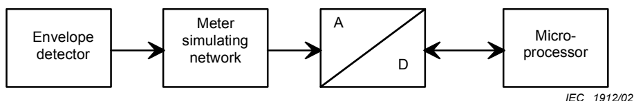
Figure 45 – Block diagram of an average detector.
