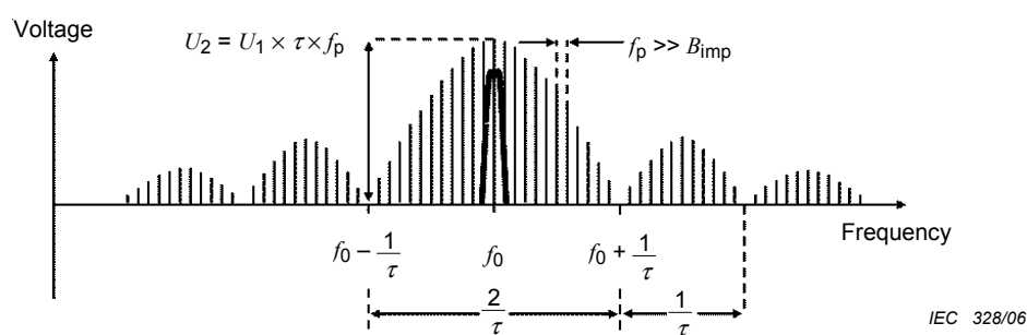
Figure E.5 – Filtering with a B_{\text{imp}} much smaller than the prf
