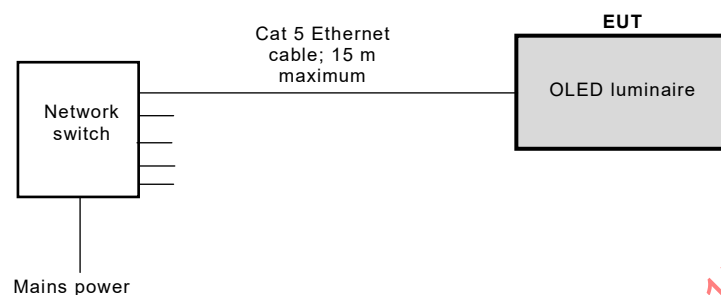
Figure D.4 – Case 4 EUT
