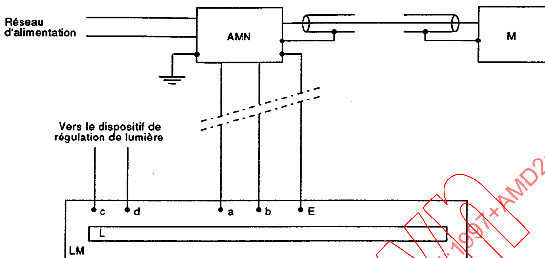
Figure 6a – Luminaires
