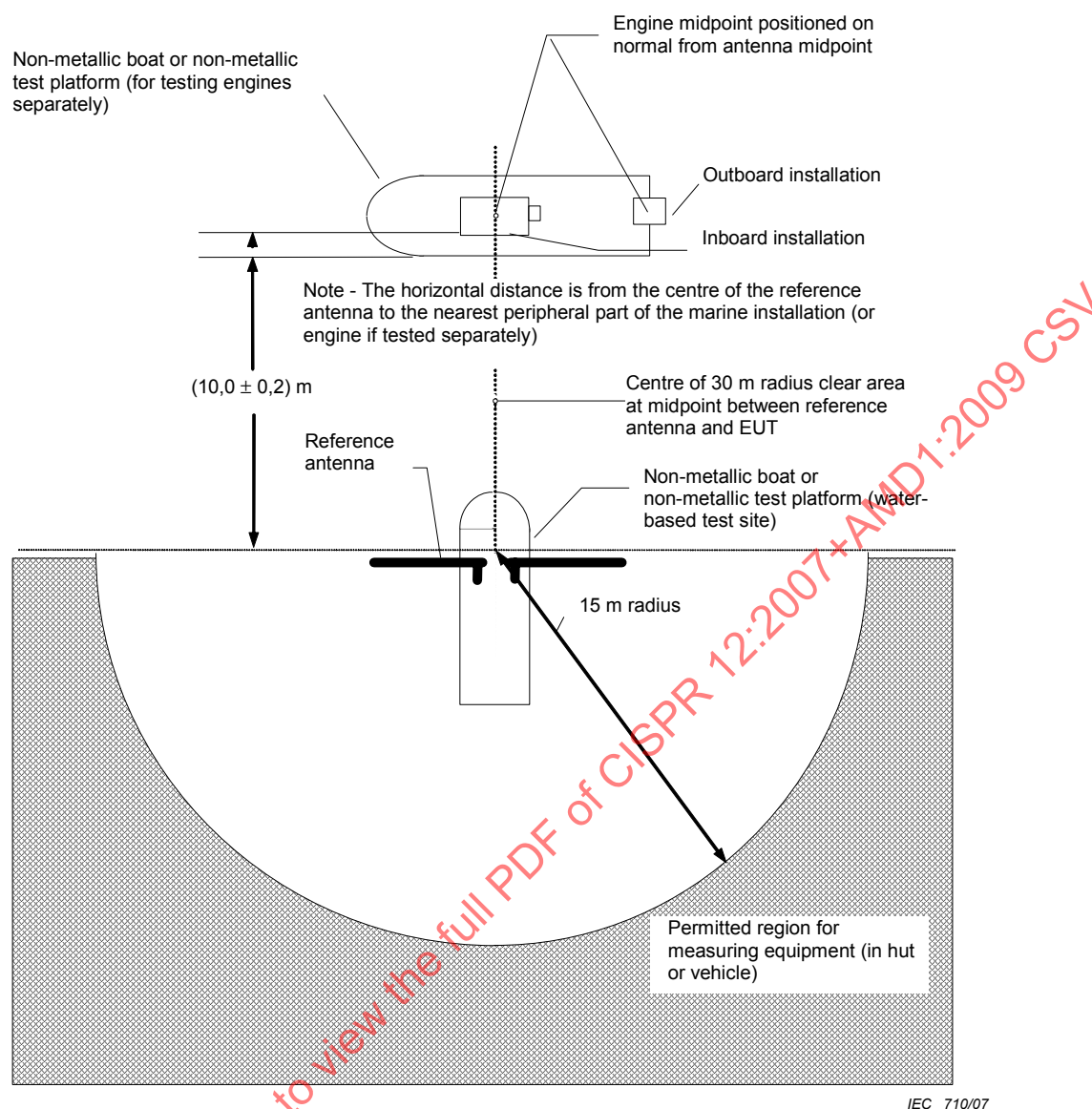
Figure 5 – Measuring site (OTS) for boats
