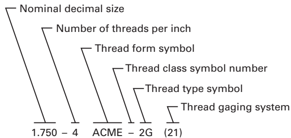
FIG. 18 ACME SCREW THREAD DESIGNATION
