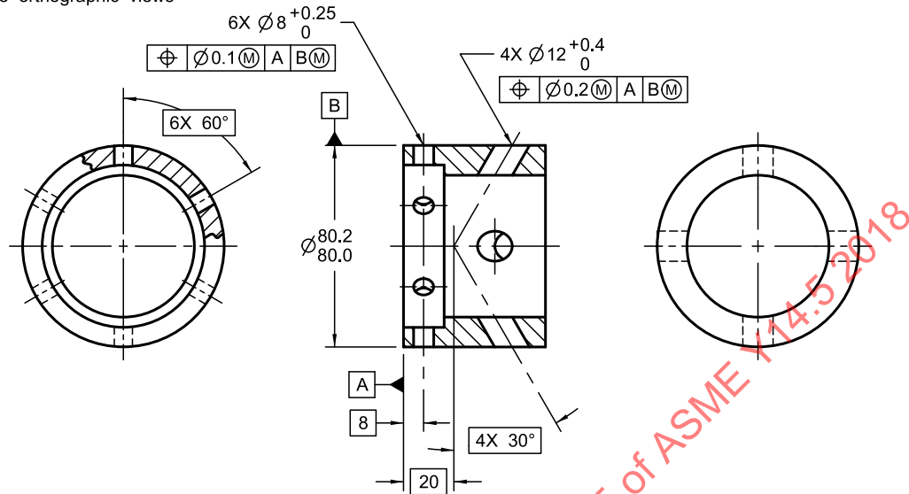
Figure 10-37 Nonparallel Holes Including Those Not Normal to the Surface
