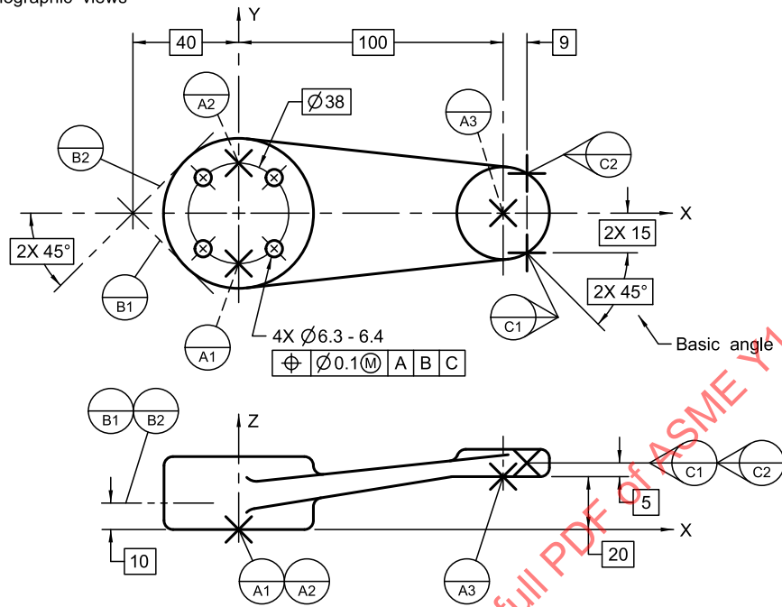
Figure 7-58 Application of Movable Datum Targets
