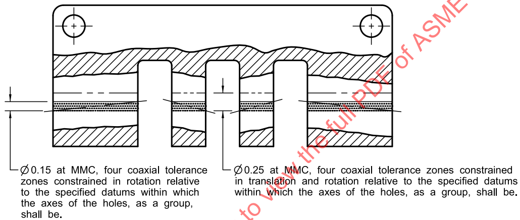
Figure 10-52 Positional Tolerancing for Multiple Features of More Than One Size
