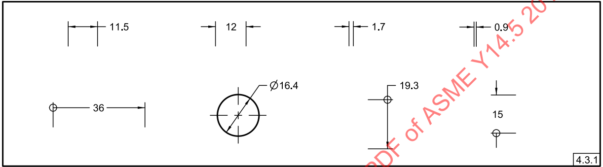
Figure 4-2 Millimeter Dimensions
