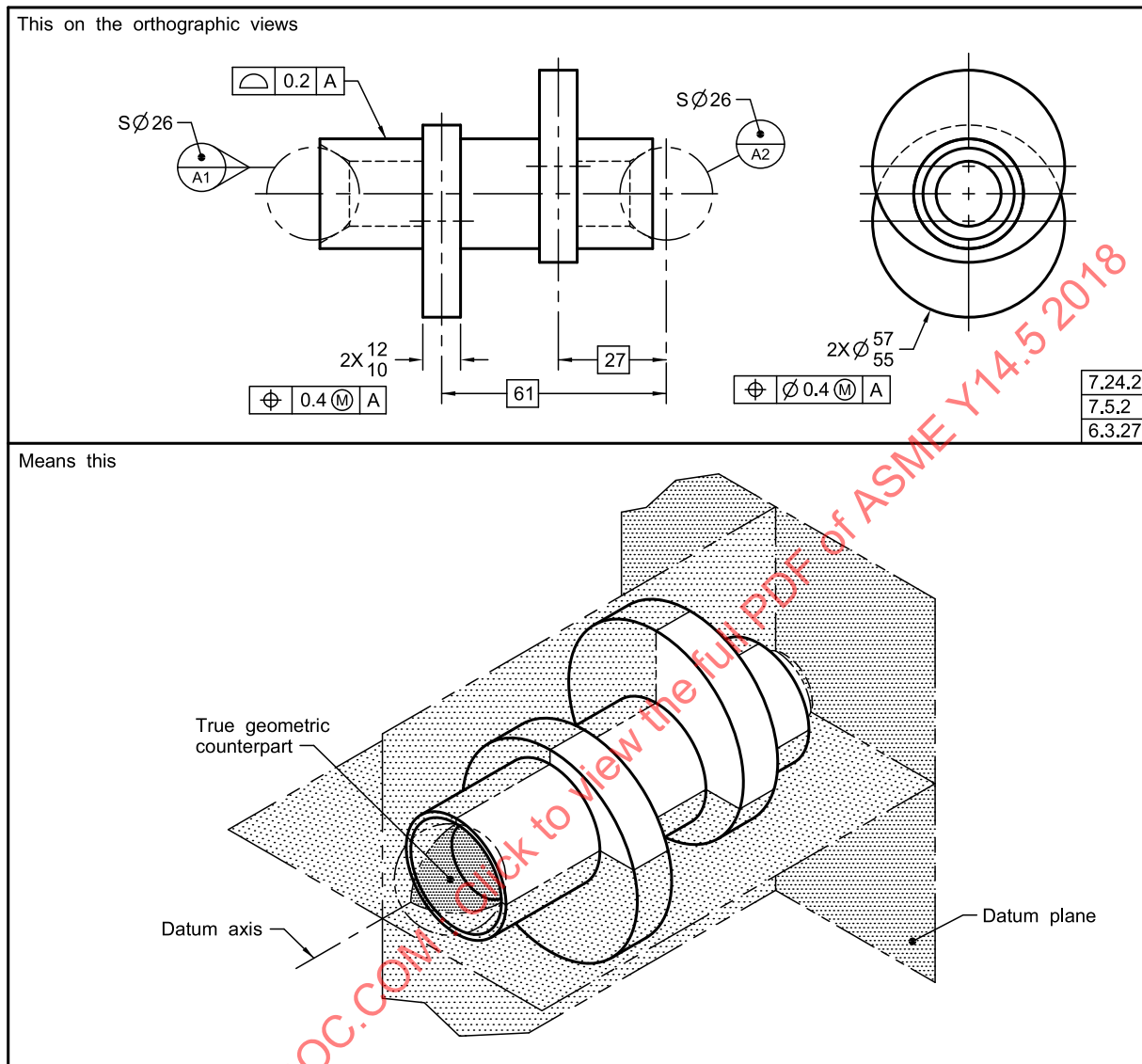
Figure 7-59 Datum Target Spheres
