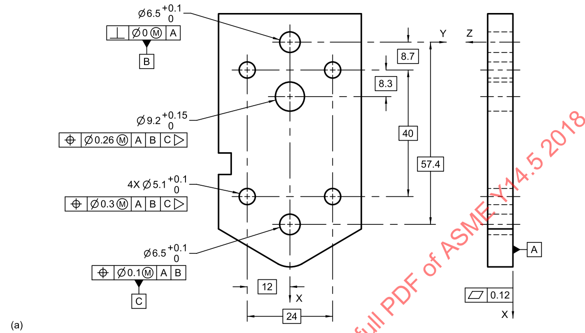
Figure 7-12 Development of a Datum Reference Frame With Translation Modifier
