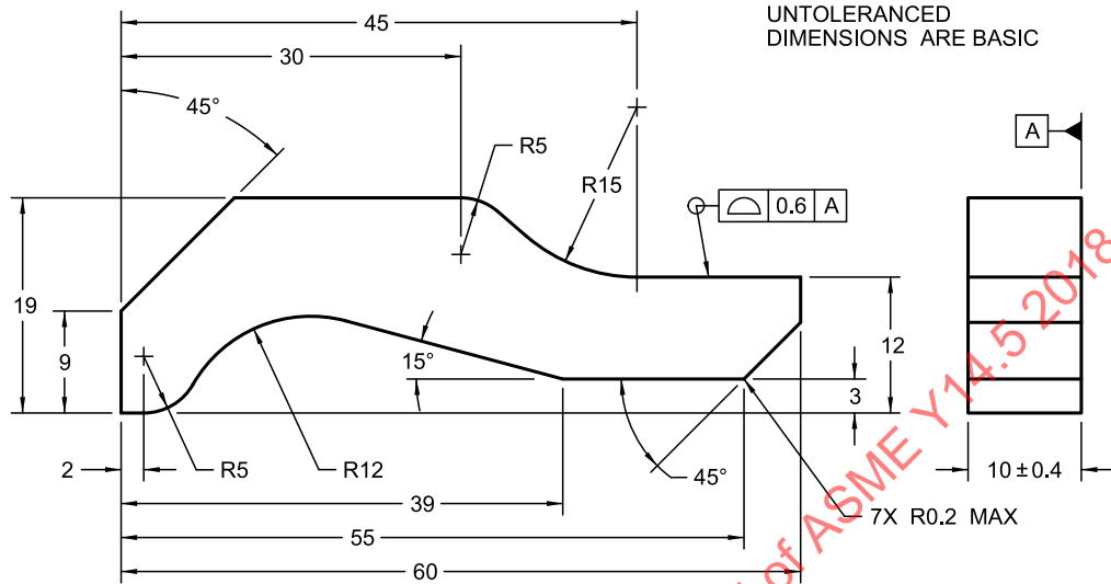
Figure 11-6 Specifying Profile of a Surface All Around
