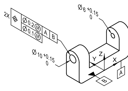
Figure 10-52 Positional Tolerancing for Multiple Features of More Than One Size
