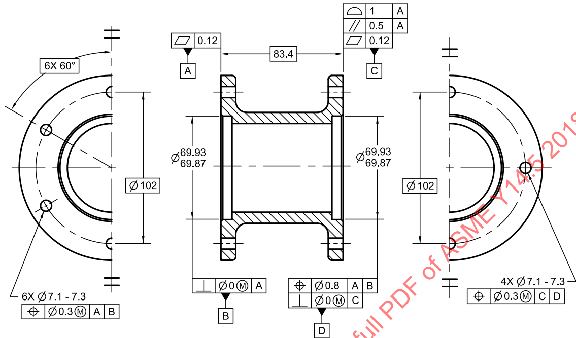
Figure 7-15 Multiple Datum Reference Frames and Their Interrelationships
