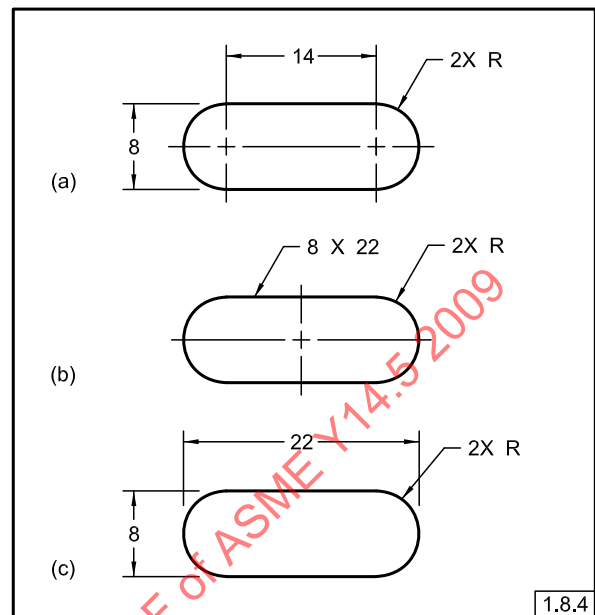
Fig. 1-29 Slotted Holes
