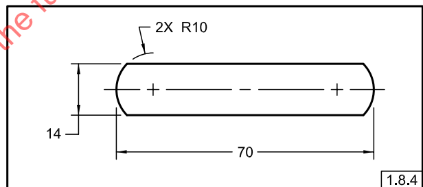
Fig. 1-31 Rounded Corners
