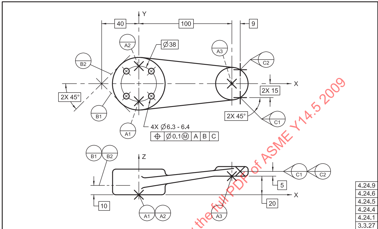
Fig. 4-47 Applications of Movable Datums
