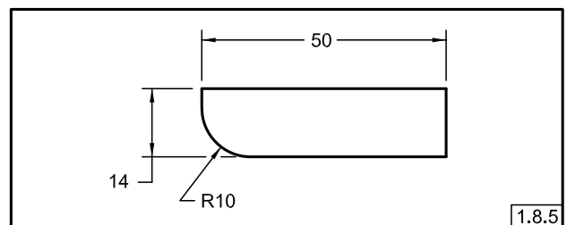
Fig. 1-31 Rounded Corners
