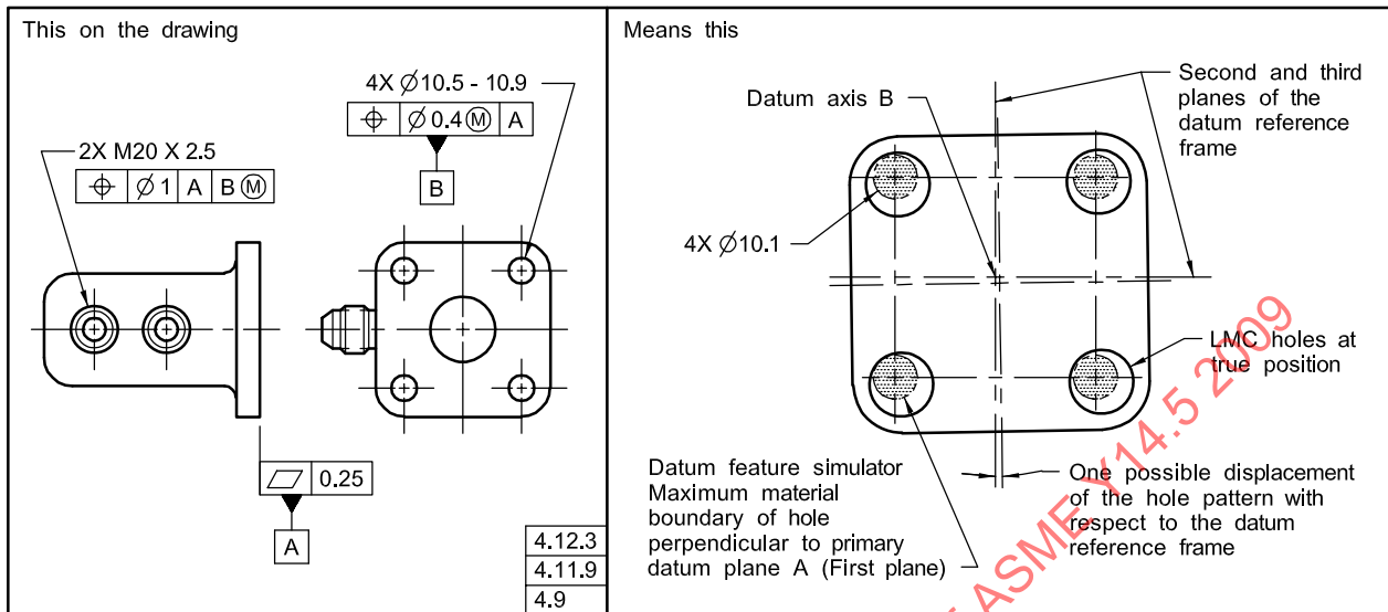
Fig. 4-26 Hole Pattern Identified as Datum
