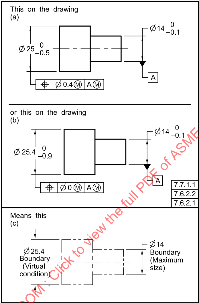
Fig. 7-56 Positional Tolerancing for Coaxiality
