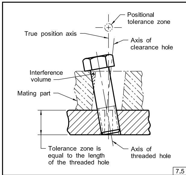
Fig. 7-19 Interference Diagram, Fastener and Hole
