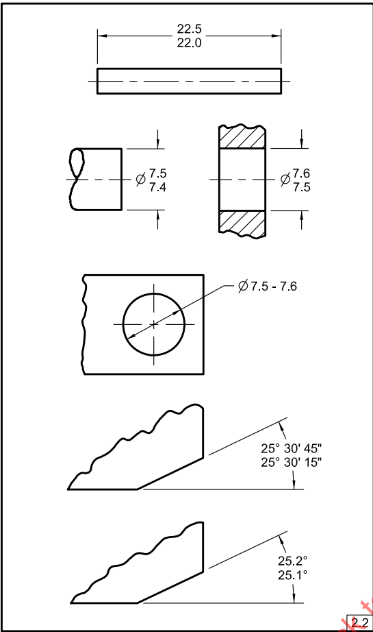
Fig. 2-1 Limit Dimensioning
