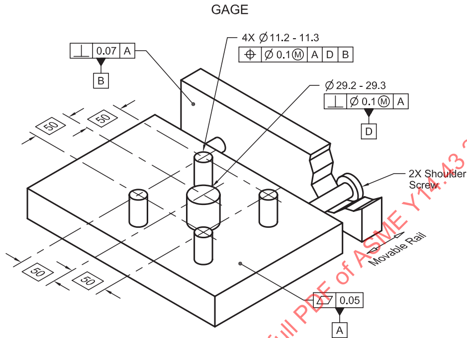
Fig. B-9 Size and Planar Datum Features (Cont'd)
