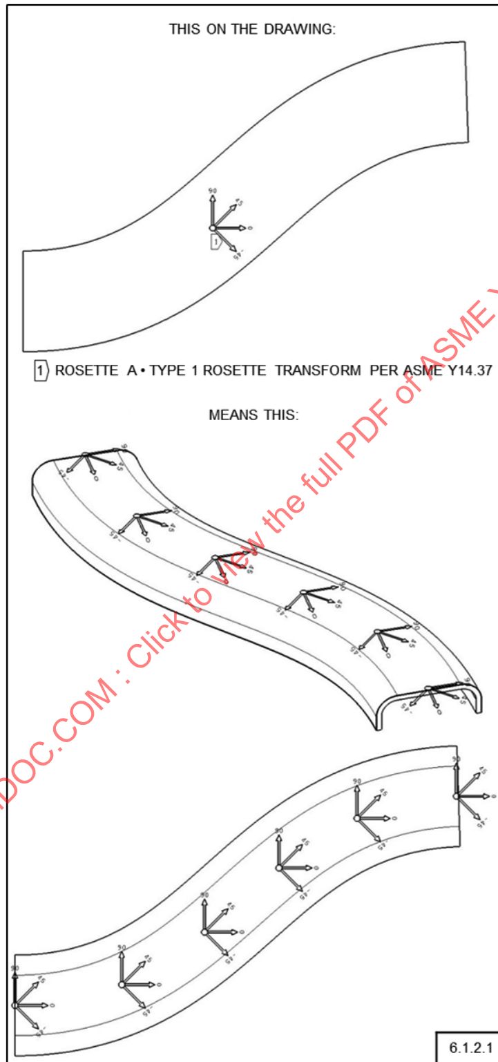
Figure 6-1 Type 1 Rosette
