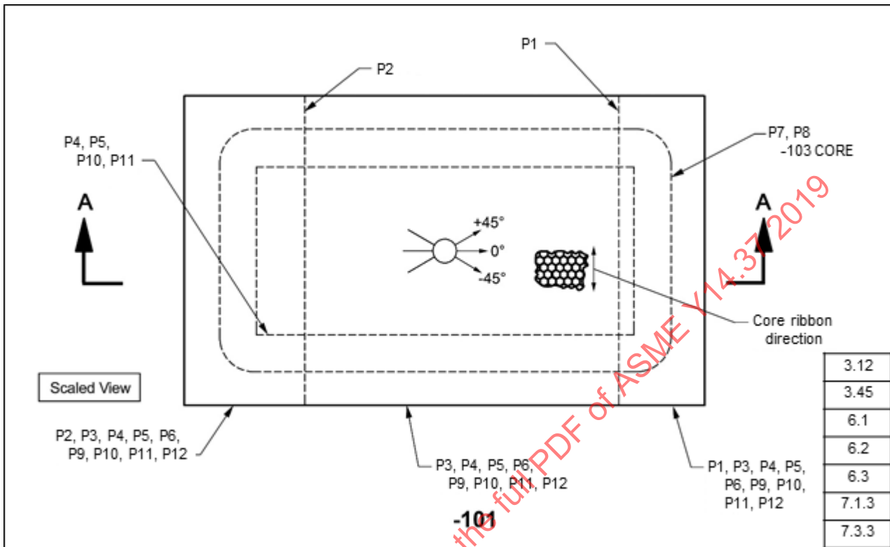
Figure 3-1 Ply Definition
