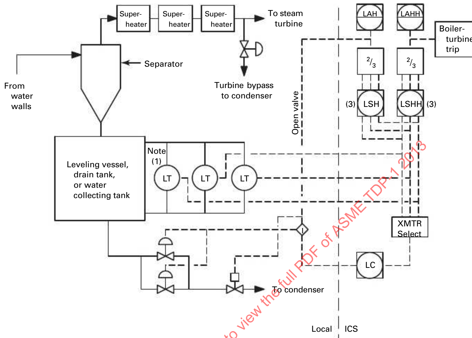
Fig. 3 Typical Leveling System Arrangement: Integrated Control System
