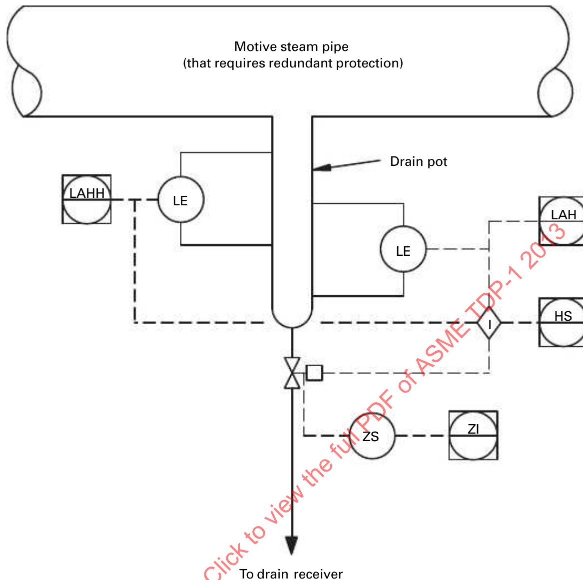
Fig. 5 Typical Drain System With Redundant Level Elements
