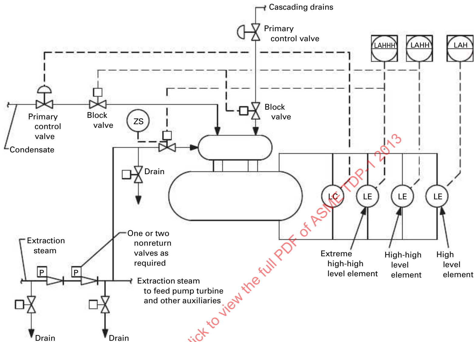
Fig. 12 Typical Deaerator Arrangement With Inlet Isolation: Local Control System
