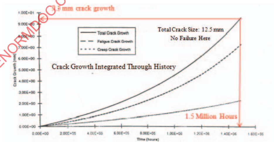
Figure 12 - Crack Growth versus Time
