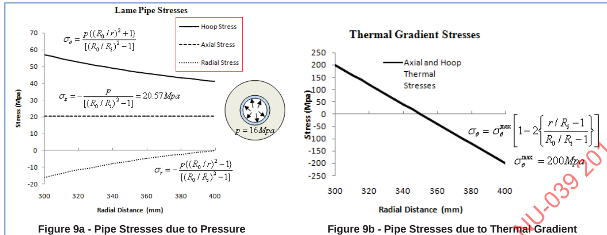
Figure 9 - Pipe Stresses
