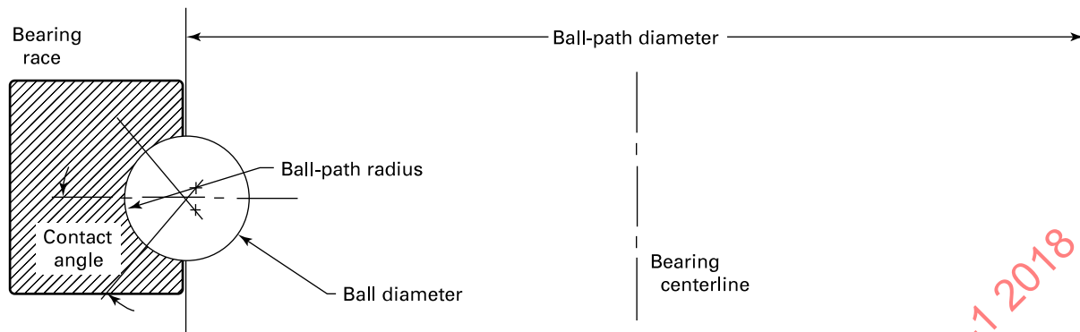
Figure 2.1-1 Single-Row Four-Point Contact Ball Bearing Definitions
