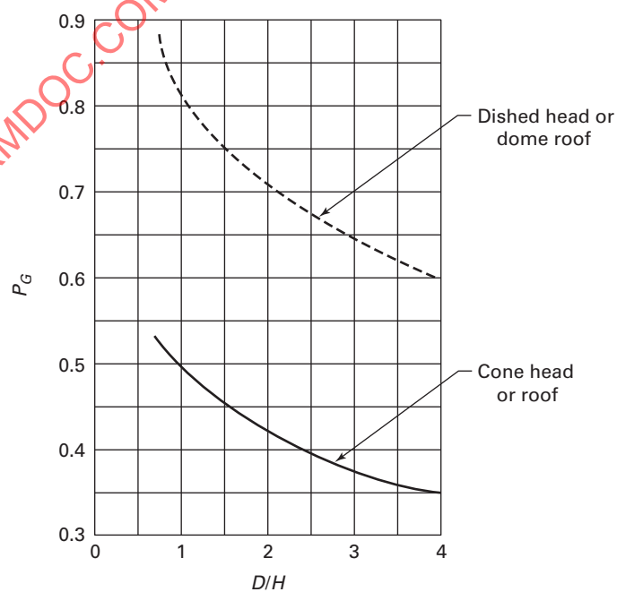
Fig. NM4-4 Uplift Coefficient, P_G
