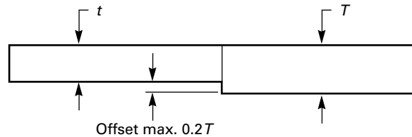
Fig. M12D-1 Maximum Offset Allowed for Joints Between Sheets With Different Thicknesses
