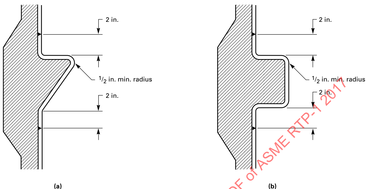
Fig. M12C-1 Support Ledges Showing Recommended Weld Locations Away From Thermoformed Bends
