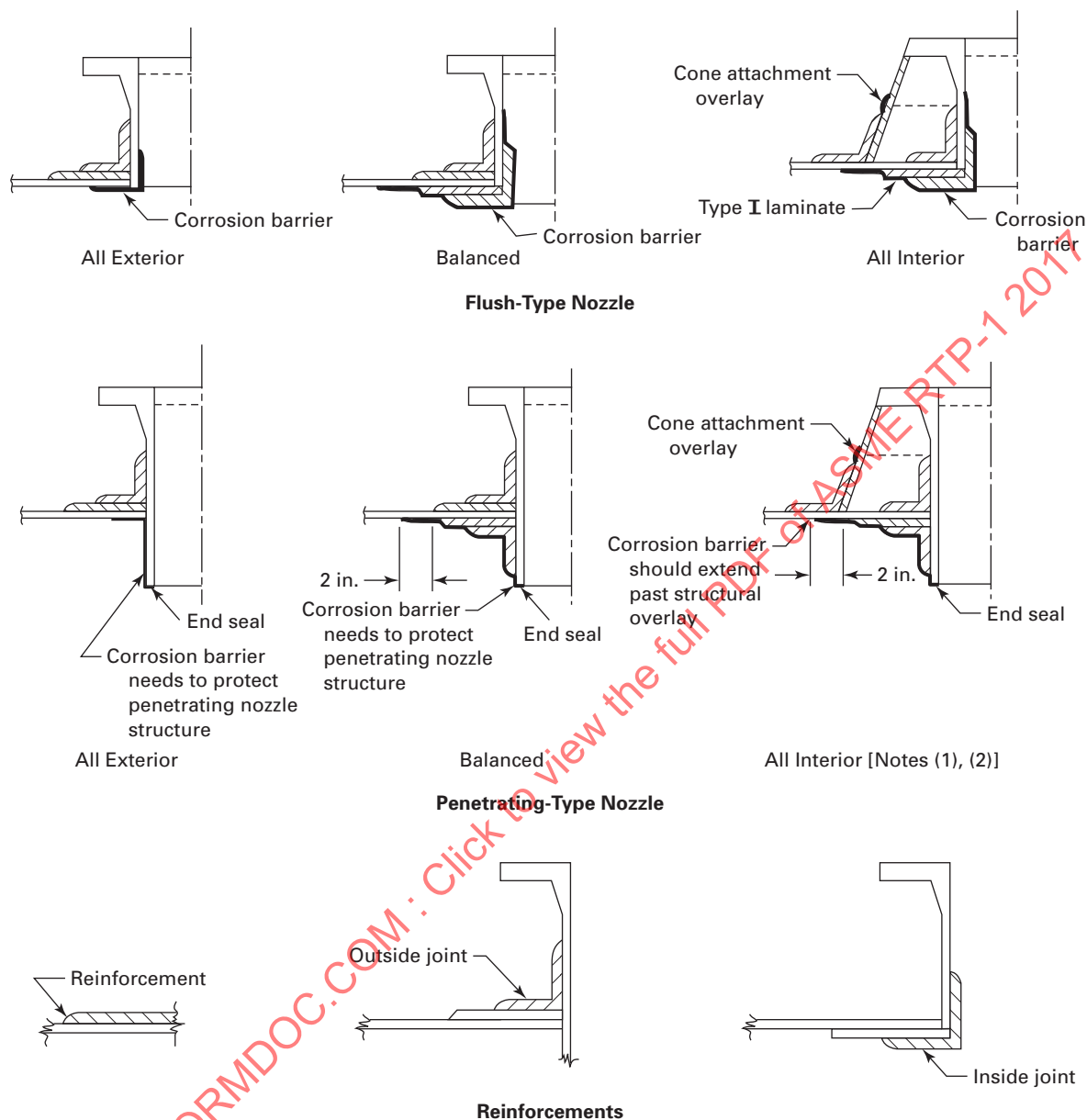
Fig. 4-12 Nozzle Installation and Cutout Reinforcement Location Alternate
