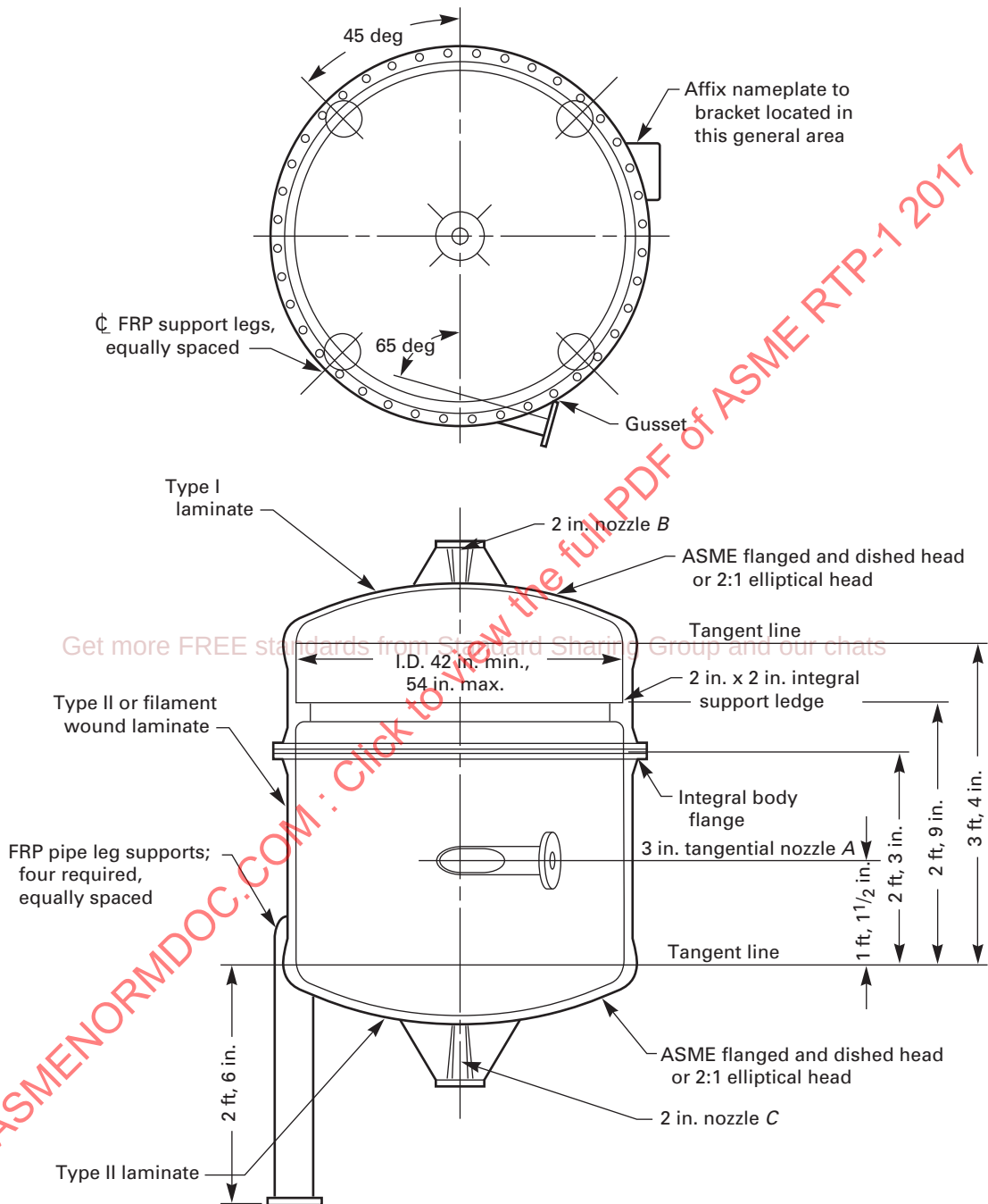
Fig. M12G-1 Dual Laminate Demonstration Vessel
