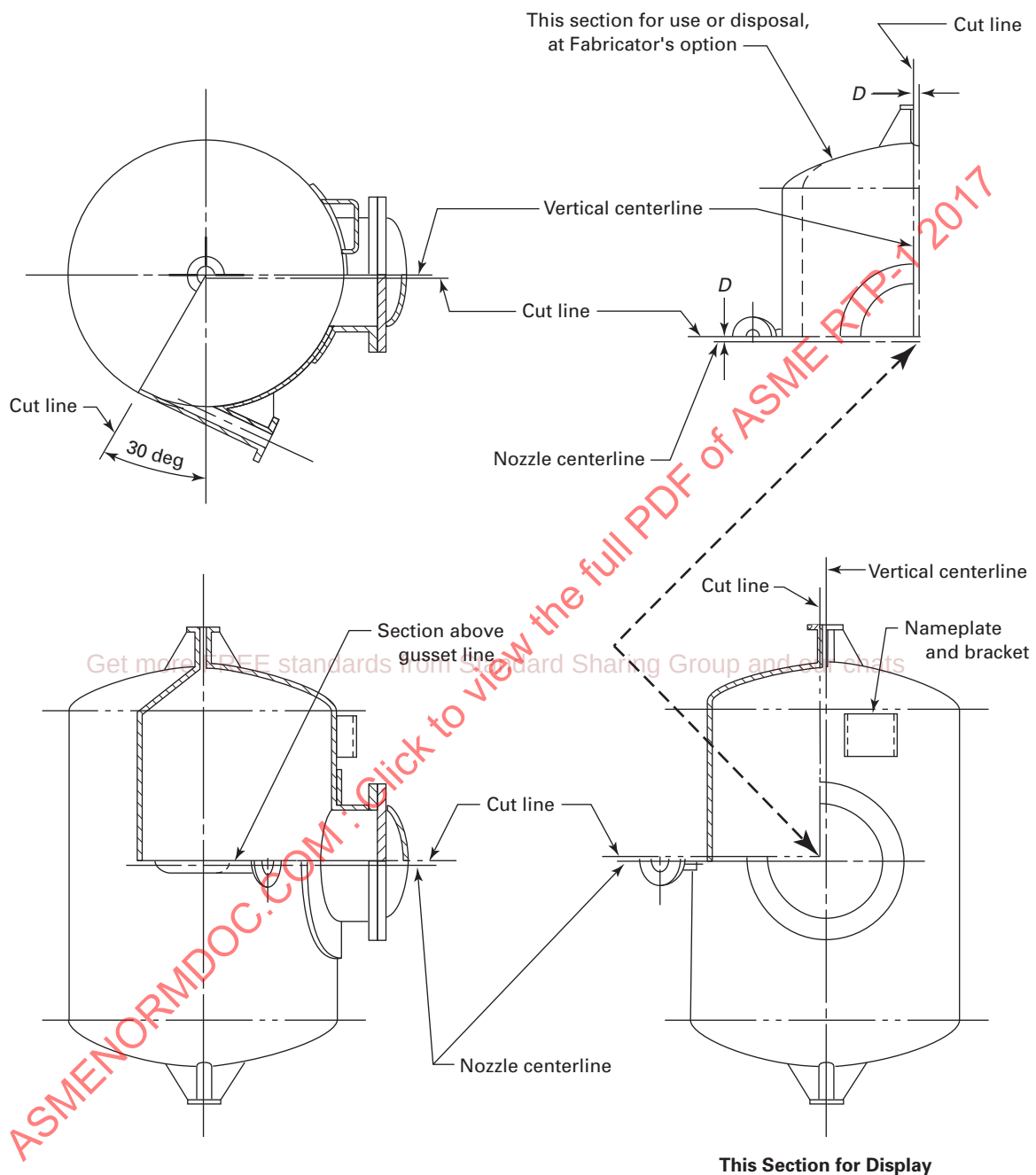
Fig. M6-2 Post-Test Sectioning of Vessel for Final Inspection and Display
