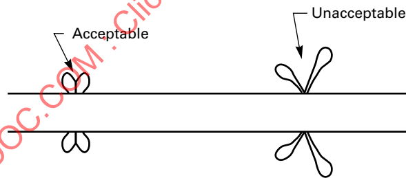
Fig. M12D-5 Butt Fusion Welds Showing Melt Flow Lines
