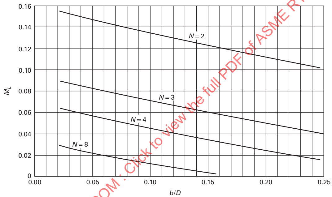
Fig. NM5-2 Moment Coefficient, M_L
