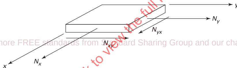
Fig. M3-2 Force Resultants
