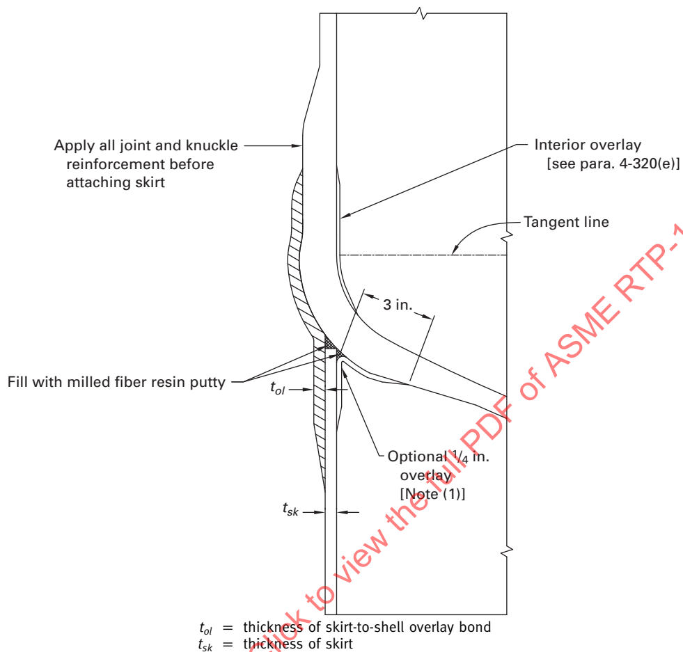
Fig. 4-8 Support Skirt Attachment Detail
