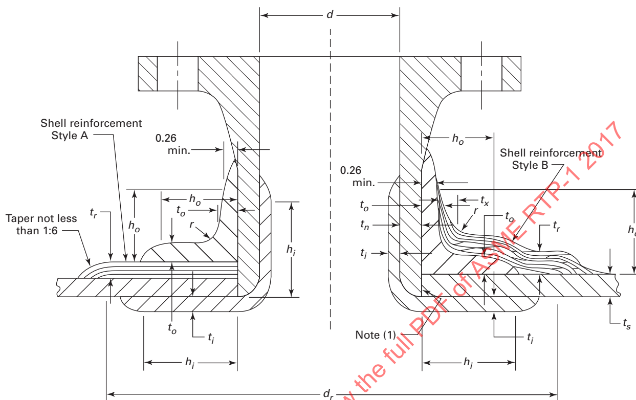
Fig. 4-4 Flush Nozzle Installation
