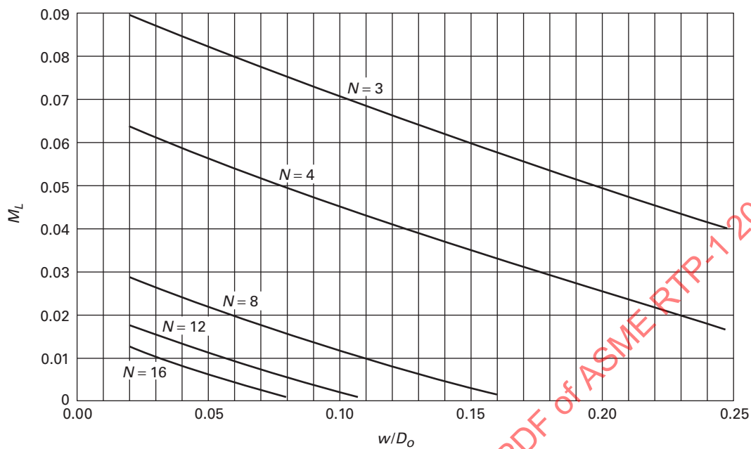
Fig. NM4-3 Moment Coefficient, M_L
