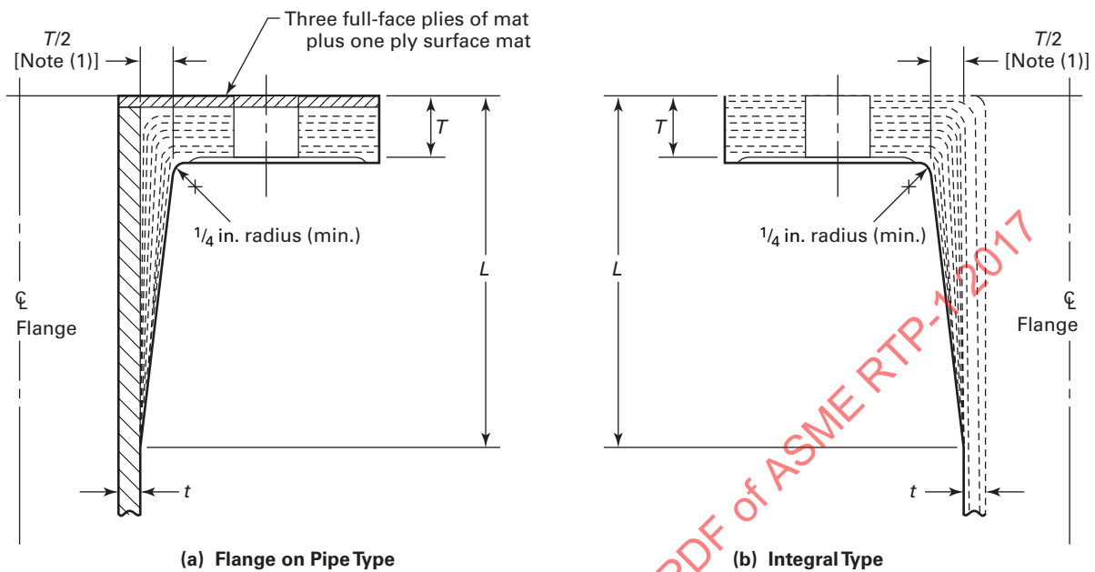
Fig. 4-11 Flanged Nozzle Lay-Up Method
