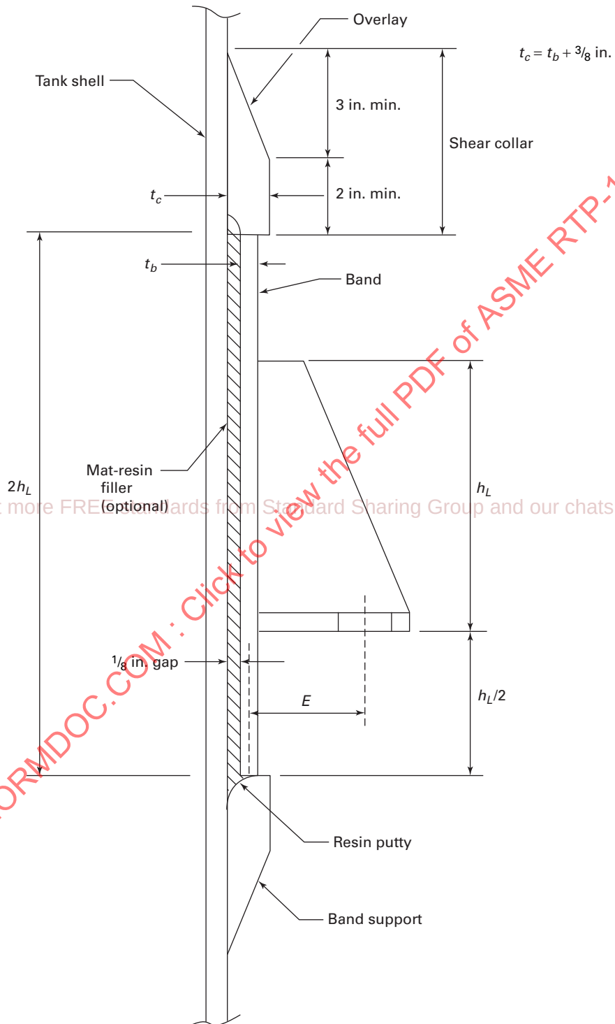
Fig. NM5-1 Lugs on Band
