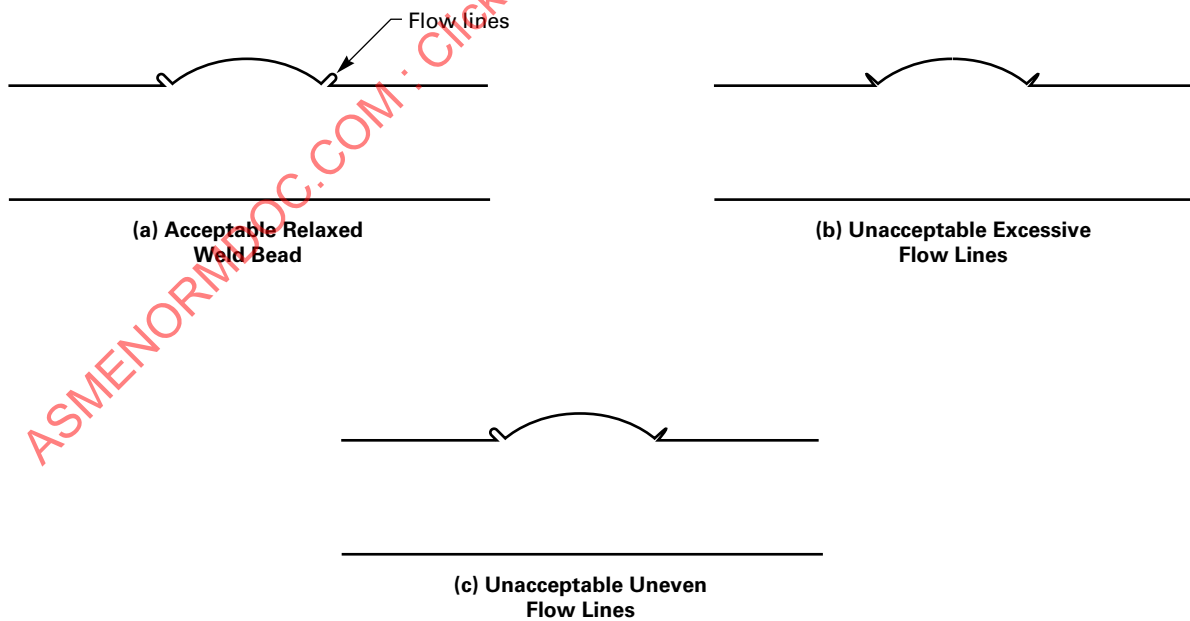
Fig. M12D-3 Illustrations of Flow Lines
