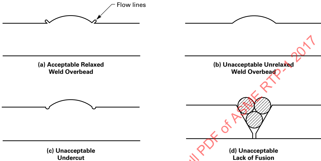
Fig. M12D-2 Visual Features of Hot Gas Welds
