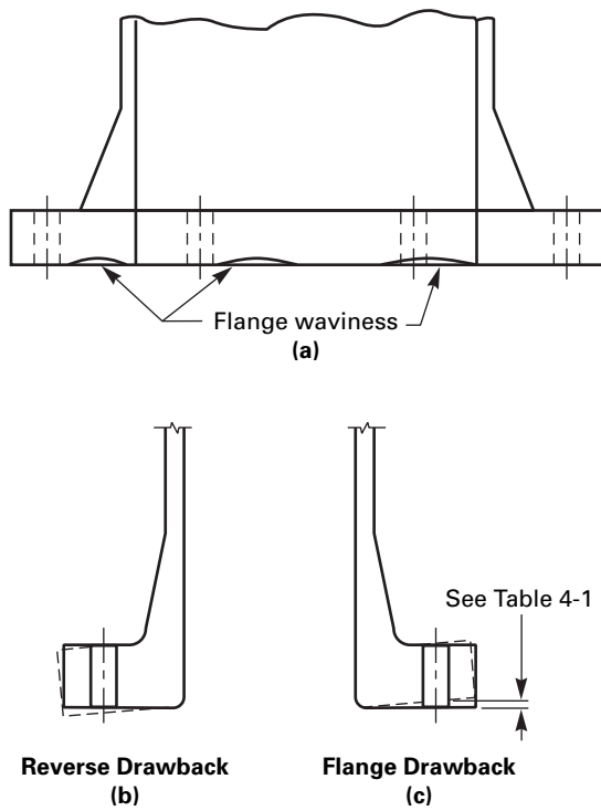
Fig. 4-14 Flange Tolerances
