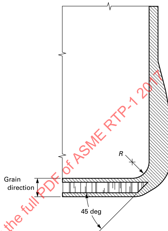
Fig. 4-15 Flat Cored Bottom Knuckle Detail
