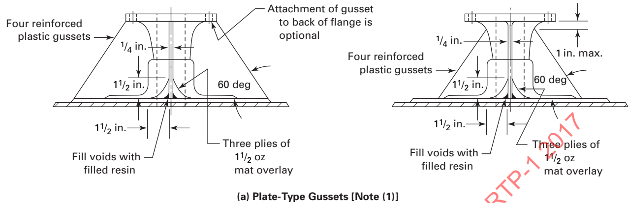
Fig. 4-13 Nozzle Gussets
