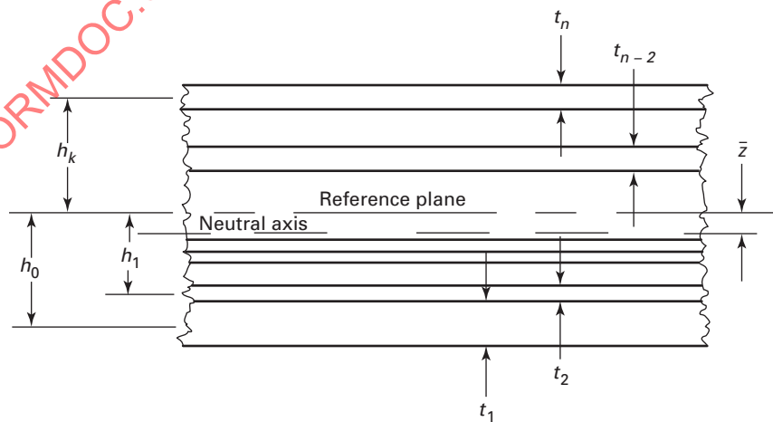
Fig. M3-3 Geometry and Notation of an n -Layered Laminate
