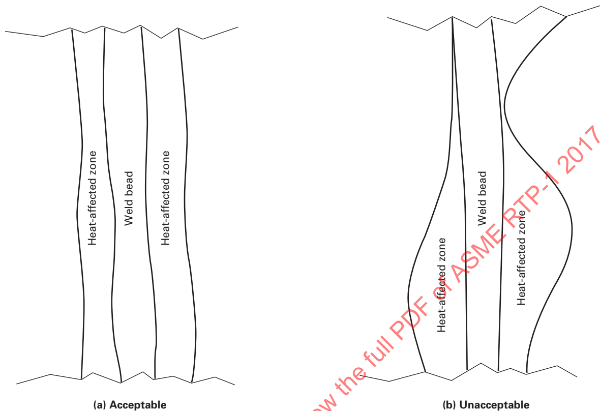
Fig. M12D-4 Heat-Affected Zone Patterns
