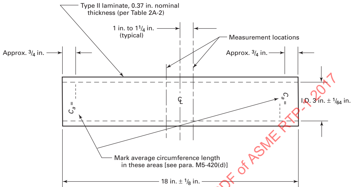
Fig. M5-1 Pipe Test Piece
