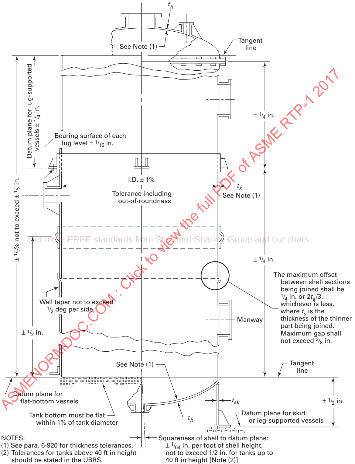
Fig. 4-9 Fabrication Tolerances
