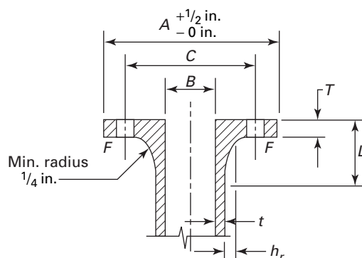
Fig. 4-10 Nozzle Flange Dimensions for Class 150 Bolting
