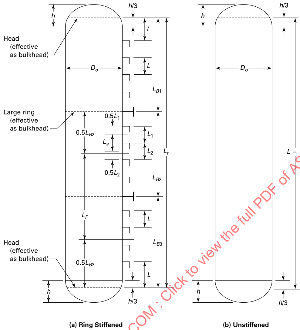
Figure 1-7.13.1-1 Geometry of Cylinders
