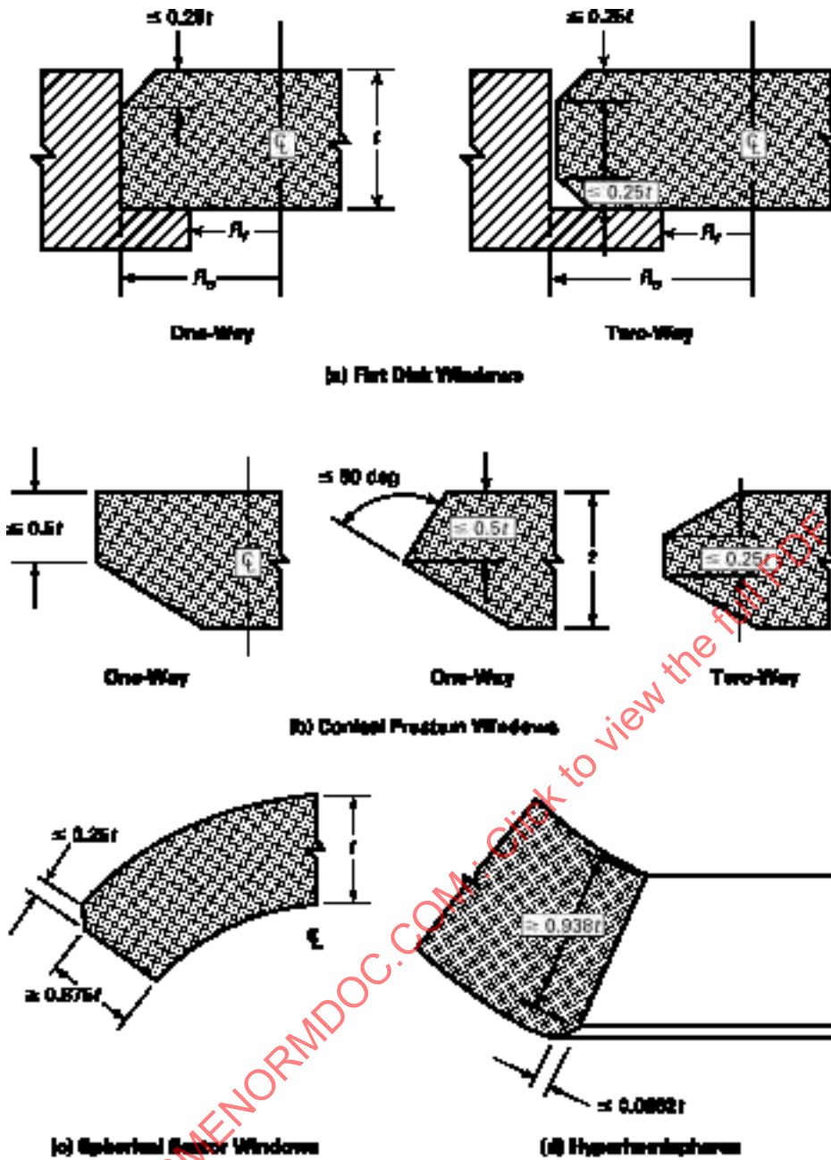
Figure 2-2.11.10-1 Bevels on Window Edges — Flat Disk Windows, Conical Frustum Windows, Spherical Sector Windows, and Hyperboloid Windows
