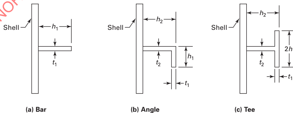
Fig. 1-7.13.1-2 Stiffener Geometry
