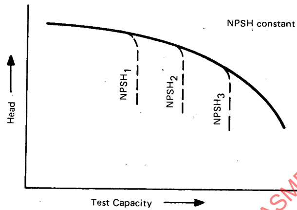
FIG. 4.44.1 CONSTANT NPSH
