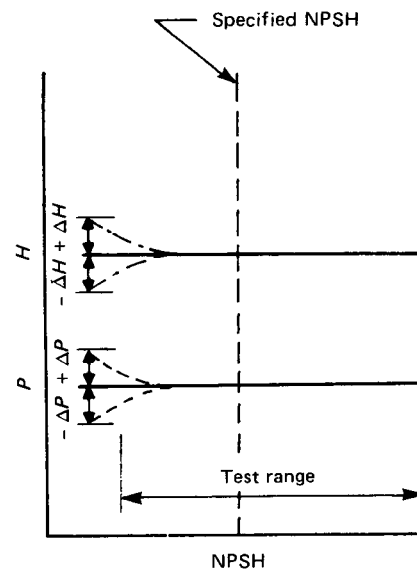
FIG. 4.43.3 CONSTANT CAPACITY
