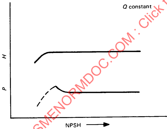
FIG. 4.43.2 CONSTANT CAPACITY
