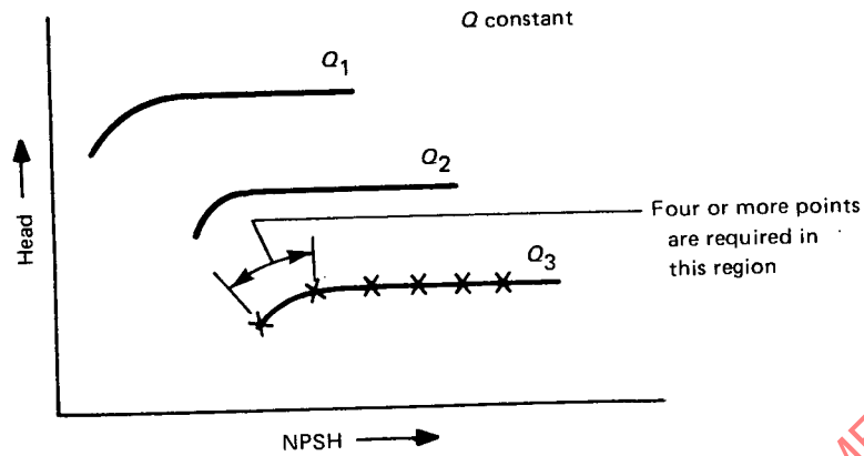
FIG. 4.43.1 CONSTANT CAPACITY
