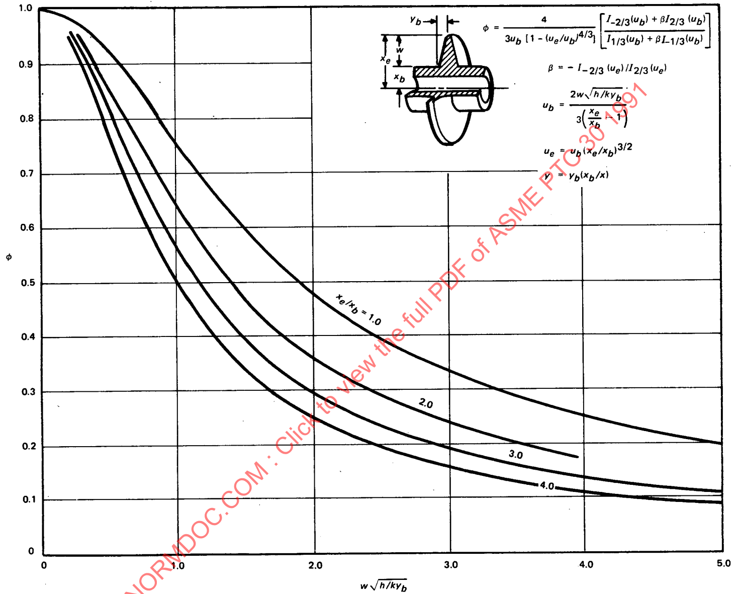
FIG. 5.13 EFFICIENCY OF ANNULAR FINNS WITH CONSTANT METAL AREA FOR HEAT FLOW
