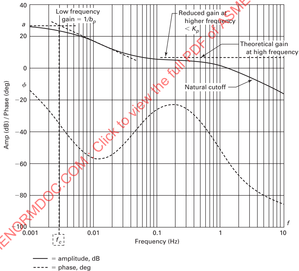
Fig. 7-3 Frequency Response Diagram
