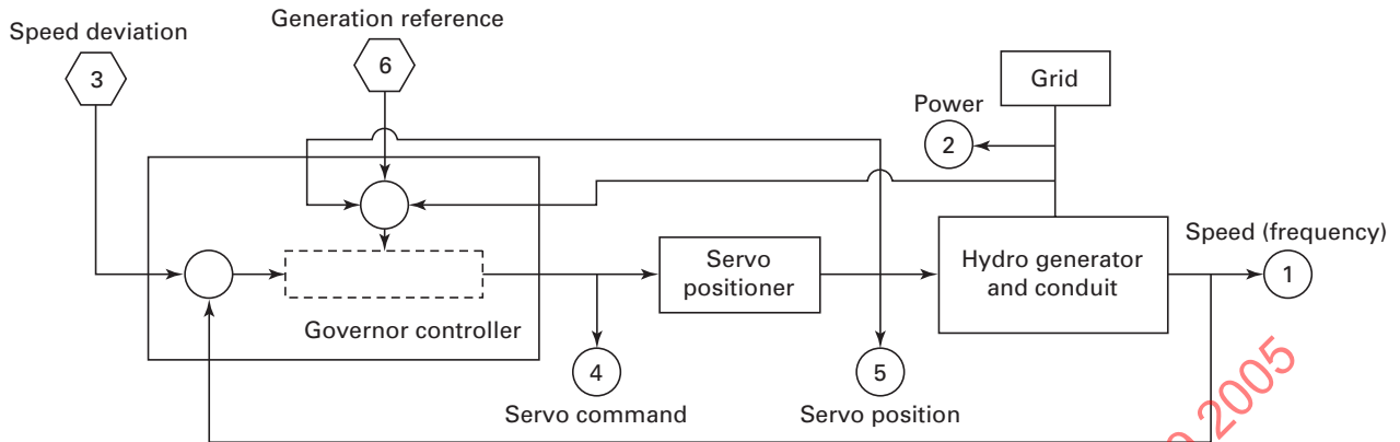
Fig. 7-2 Frequency Response Inputs and Outputs
