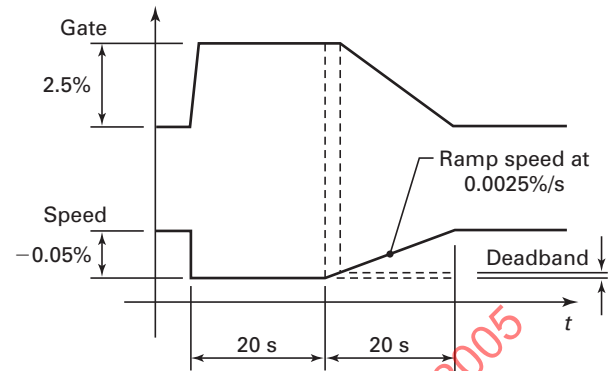
Fig. 4-2 Speed Deadband
