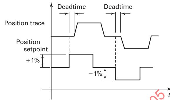
Fig. 4-4 Position Deadtime
