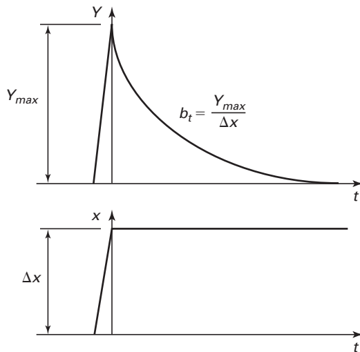
Fig. 4-1 Temporary Droop
