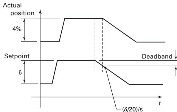
Fig. 4-3 Position Deadband
