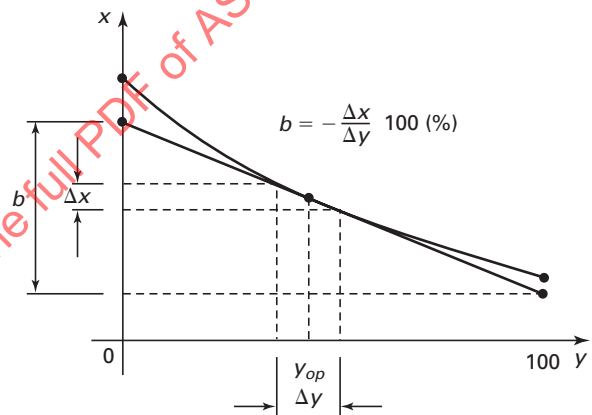
Fig. 2-7 Speed Droop
