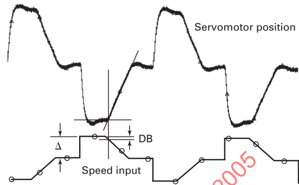
Fig. 5-1 Speed Deadband (Sample Test Plots)
