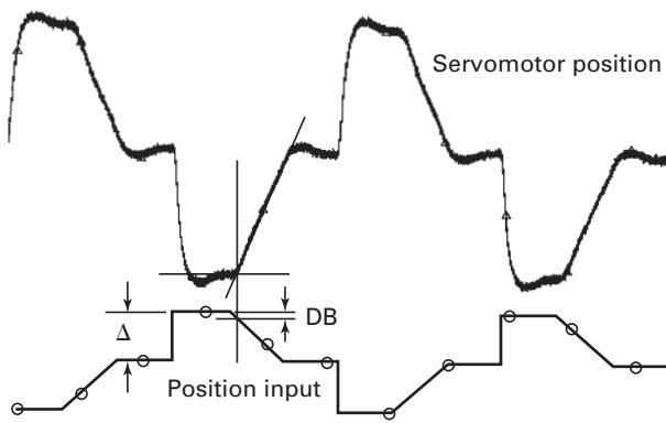
Fig. 5-3 Position Deadband (Sample Test Plots)
