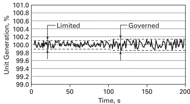
Fig. 5-7 Steady-State Power Band
