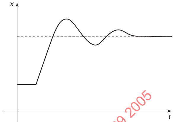
Fig. 5-8 Step Response
