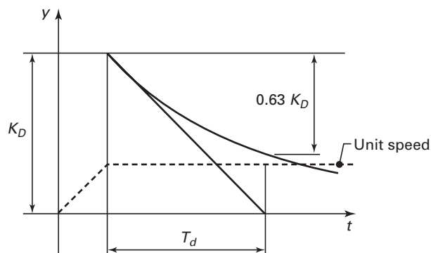
Fig. 2-4 Derivative Gain
