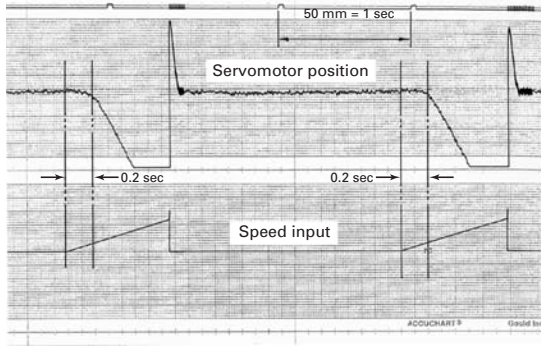
Fig. 5-2 Speed Deadtime
