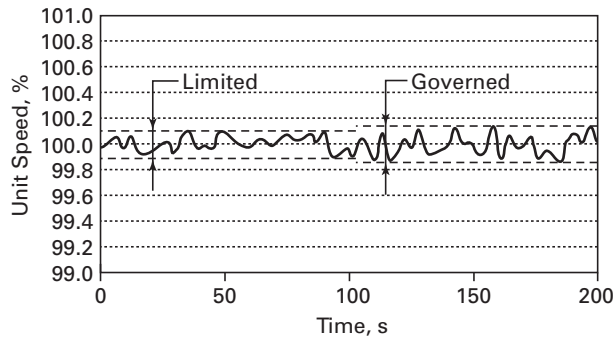
Fig. 5-6 Steady-State Speed Band
