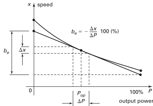
Fig. 2-5 Power Droop
