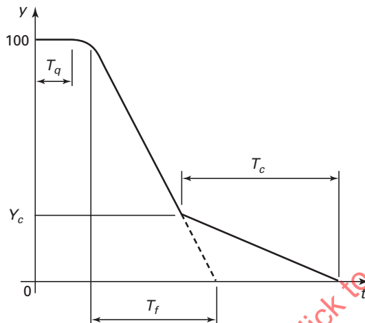
Fig. 2-6 Servomotor Time
