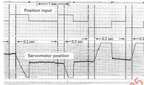
Fig. 5-4 Position Deadtime (Sample Test Plots)
