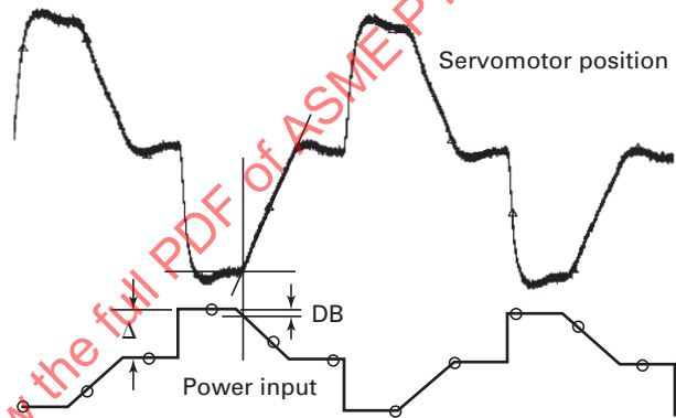
Fig. 5-5 Power Deadband
