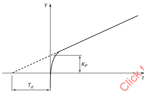
Fig. 2-1 Damping Time Constant
