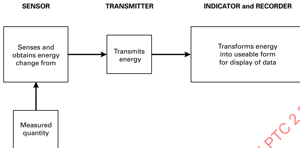
FIG. 2.2 MEASURING SYSTEM
