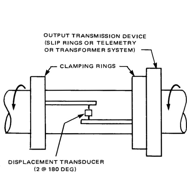
FIG. 21 MECHANICAL TYPE: ANGULAR DISPLACEMENT TORQUEMETER
