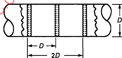
(e) Multi-Tube Type Equalizer and Straightener
