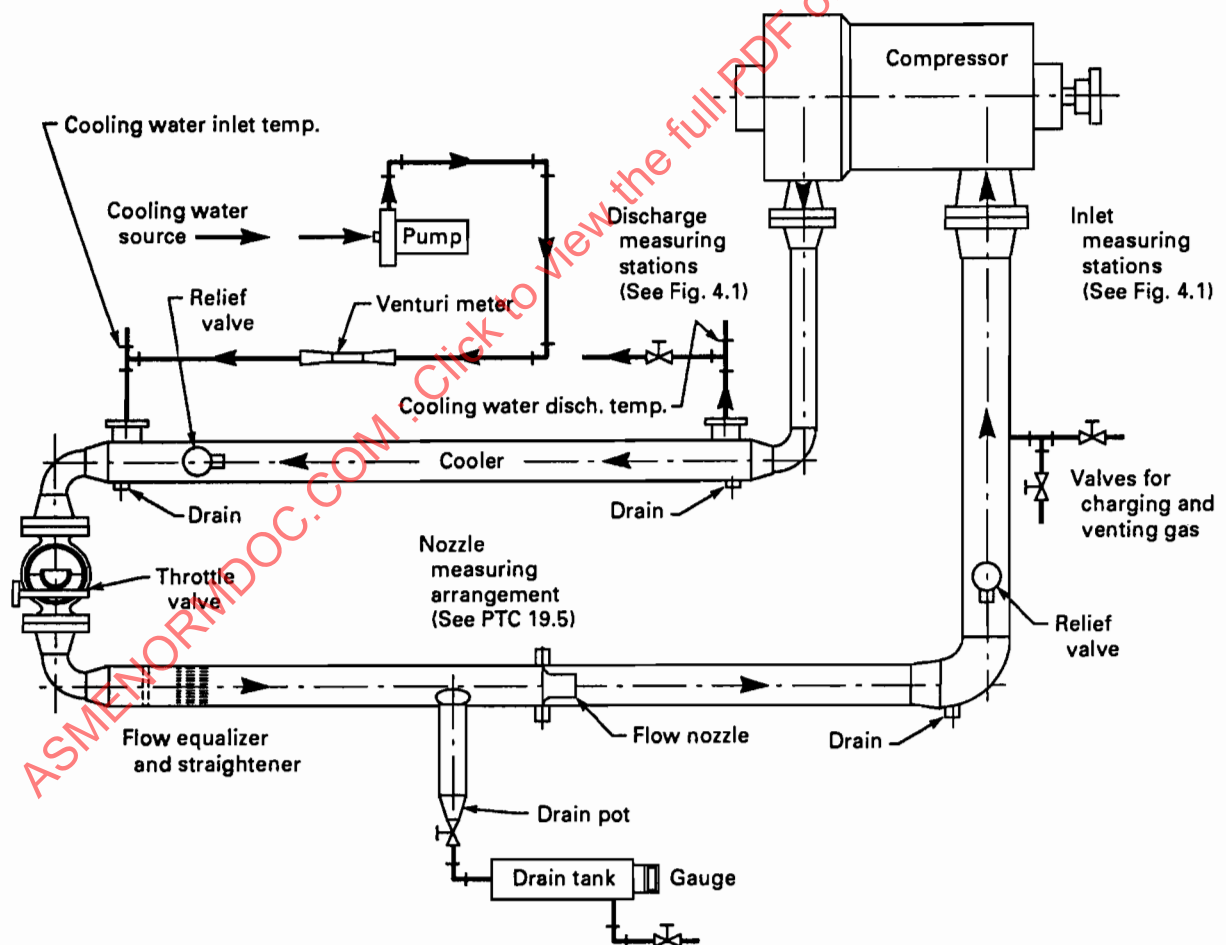
FIG. 4.6 TYPICAL CLOSED LOOP
