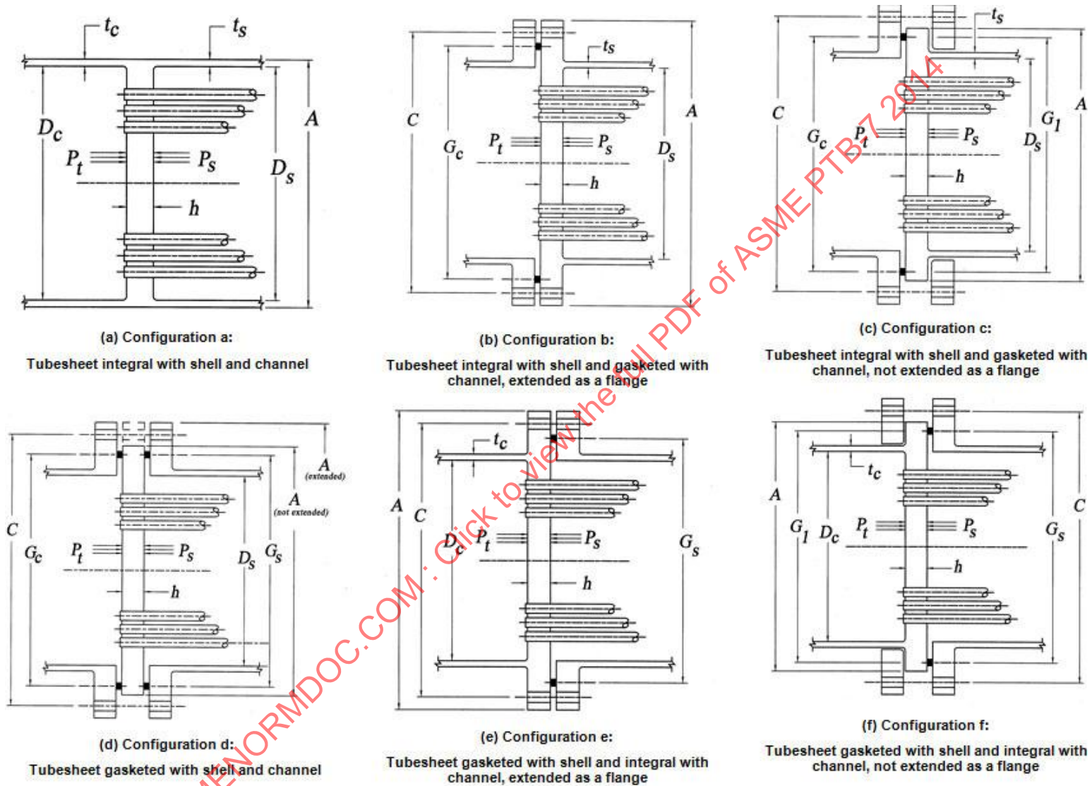
Figure 2 — Tubesheet Configurations
