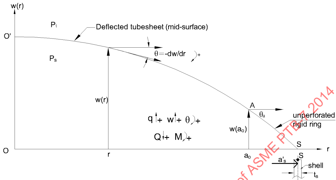
Figure 45 — TS Displacement
