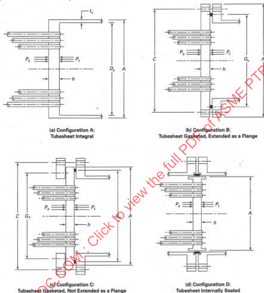
Figure 38 — Floating Tubesheet Configurations
