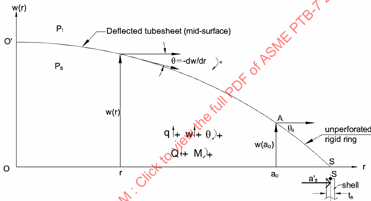
Figure 21 — TS Displacement
