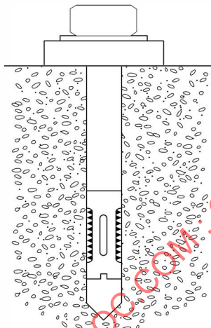
Figure 308-4.3.2-1 Sleeve Anchor
