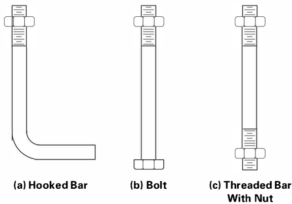
Figure 308-1.3-1 Anchors
