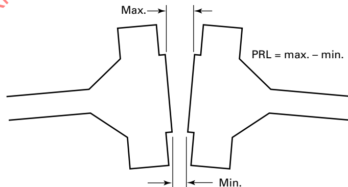
Figure E-2-3 Parallelism
