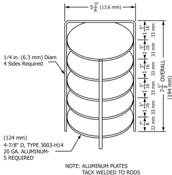
FIG. 2 SSG Samples Sintering Rack
