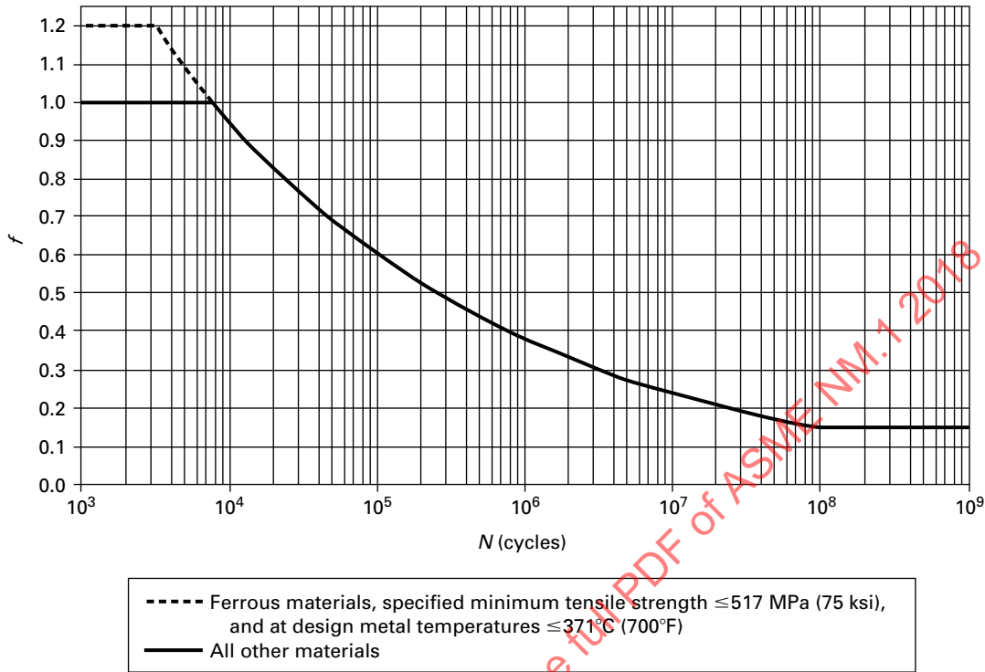
Figure 7-4.4.4.4-1 Stress Range Factor, f
