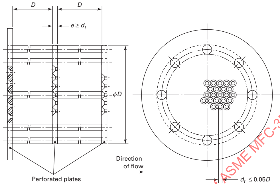
Fig. 1C-5 Sprengle Flow Conditioner
