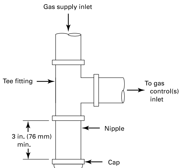
Figure CG-1 Sediment Trap
