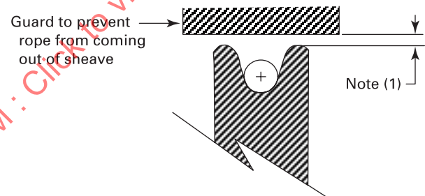
Fig. 4-2.7-1 Sheave Gap
