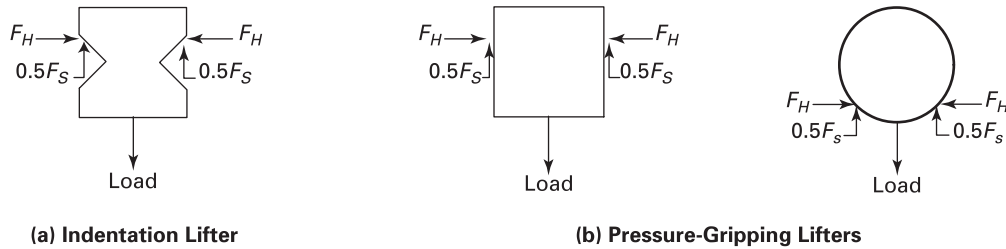
Fig. 4-9.2-1 Illustration of Holding and Support Forces
