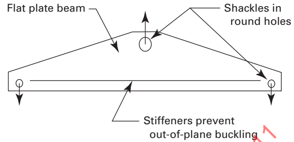
Fig. C3-4 Stiffened Plate Lifting Beam
