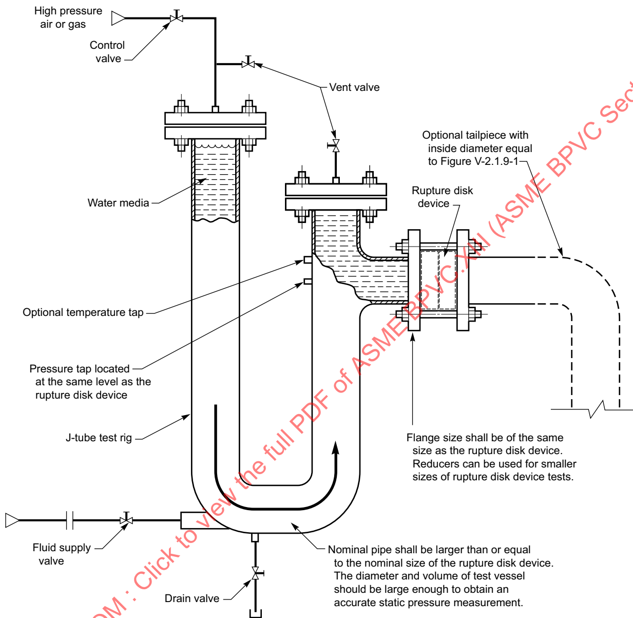
Figure V-2.2.10.1-1 Recommended Arrangement for Conducting Opening Test on Non-reclosing Pressure Relief Devices With Incompressible Fluids
