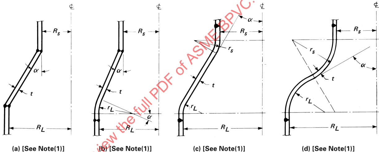
Figure UG-36 Large Head Openings — Reverse-Curve and Conical Shell-Reducer Sections
