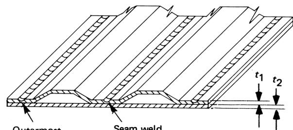
(a) Seam Welded
