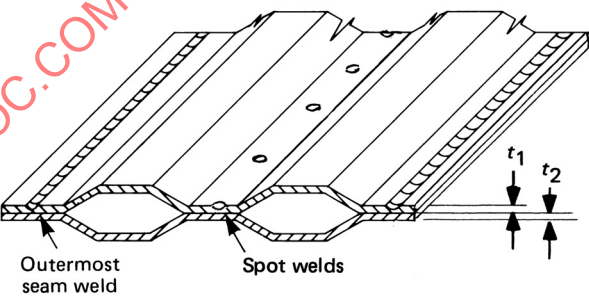
(b) Spot Welded
