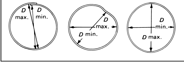
Figure UG-80.2 Example of Differences Between Maximum and Minimum Inside Diameters in Cylindrical, Conical, and Spherical Shells
