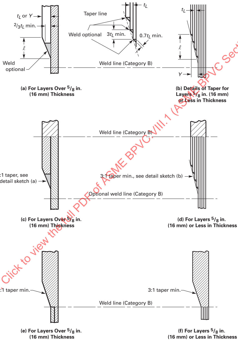
Figure ULW-17.1 Transitions of Layered Shell Sections
