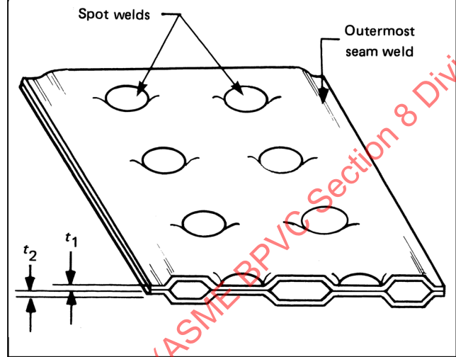
Figure 17-2 Two Dimpled Plates
