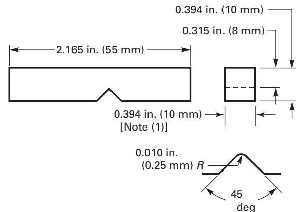
Figure UG-84 Simple Beam Impact Test Specimens (Charpy Type Test)
