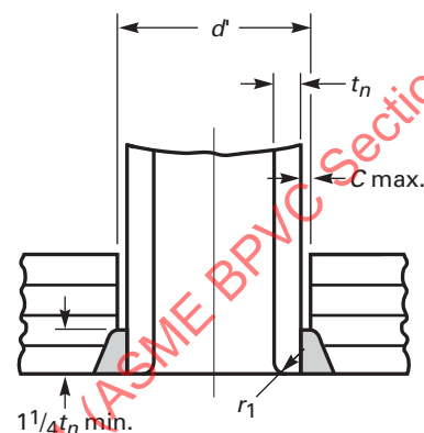
(j) [See Note (1)]
