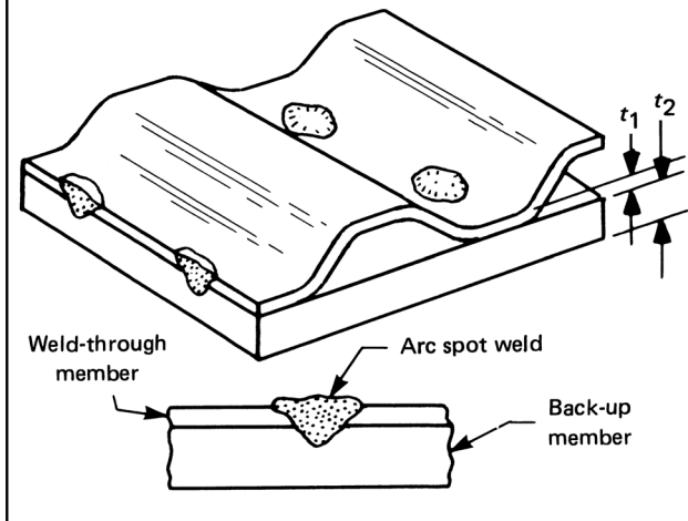
Figure 17-4 Arc-Spot-Welded Two-Layer Assembly
