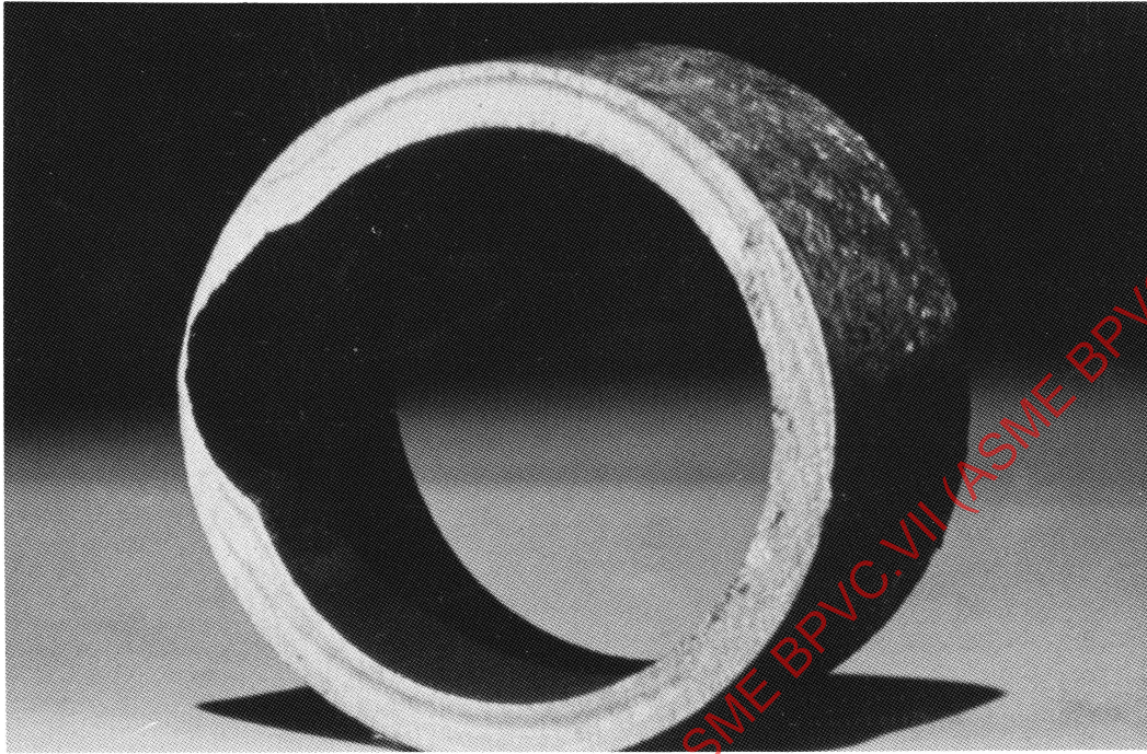
Figure 200.5.3-1 Caustic Gouge-Type Attack on Boiler Tube
