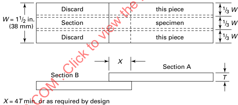
Figure QB-462.4 Lap Joint Section Specimen (See QB-181)
