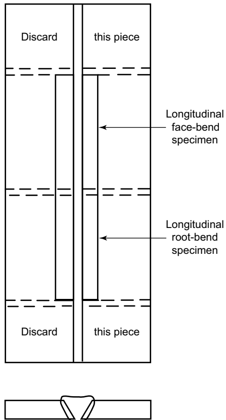
(23) Figure QW-463.2(c) Plates — Longitudinal Performance Qualification
