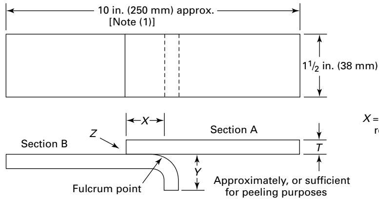
Figure QB-462.3 Lap Joint Peel Specimen
