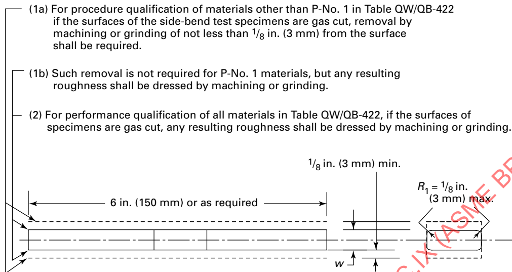
Figure QW-462.2 Side Bend
