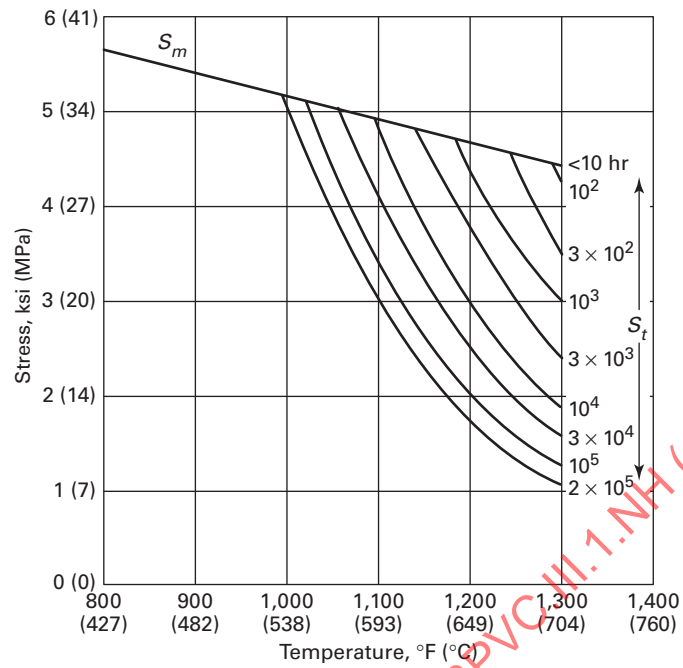
Figure NH-I-14.13A S_{mt} — Allowable Stress Intensity, Type 304 SS, Bolting
