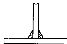
Figure NF-3626(a)-1 Additional Permissible Welded Joints for Class 1 Piping Supports
