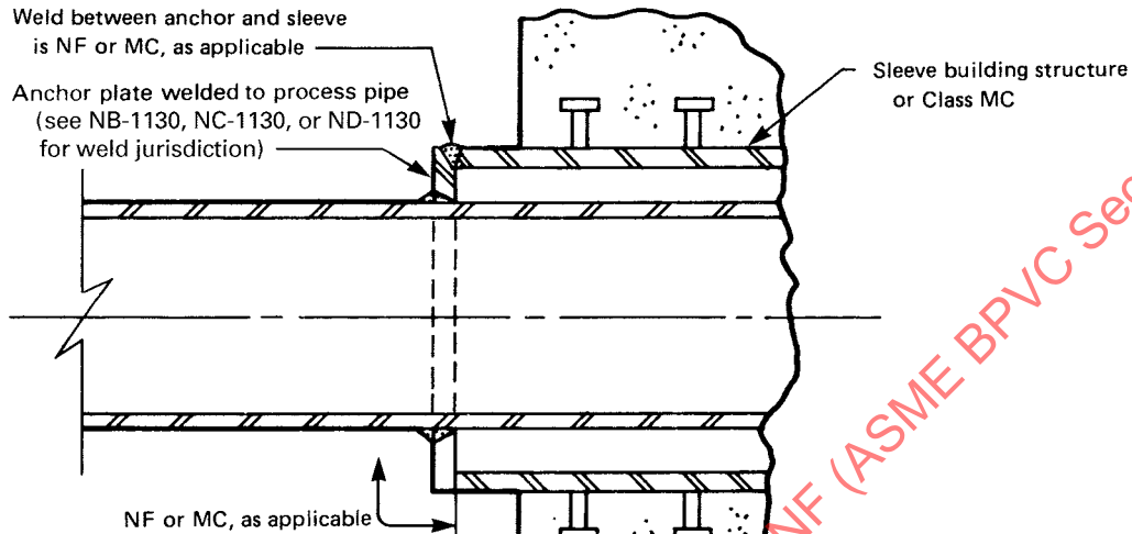
Figure NF-1132-1 Typical Examples of Jurisdictional Boundaries Between Supports and the Building Structure (Cont'd)
