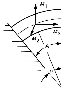
Figure NB-3686.2-1
