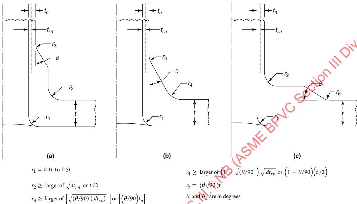
Figure NB-3339.1(b)-1 Examples of Acceptable Transition Details
