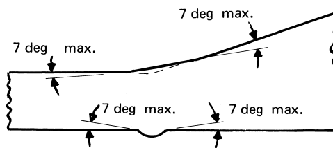
Figure NB-3683.1(c)-1
