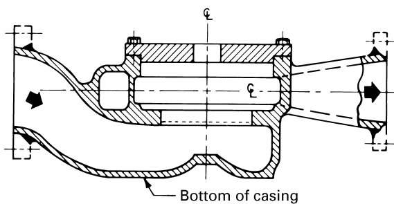
Figure NB-3441.3-1 Type C Pump
