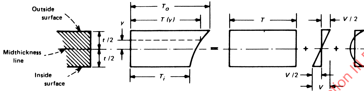
Figure NB-3653.2(b)-1 Decomposition of Temperature Distribution Range
