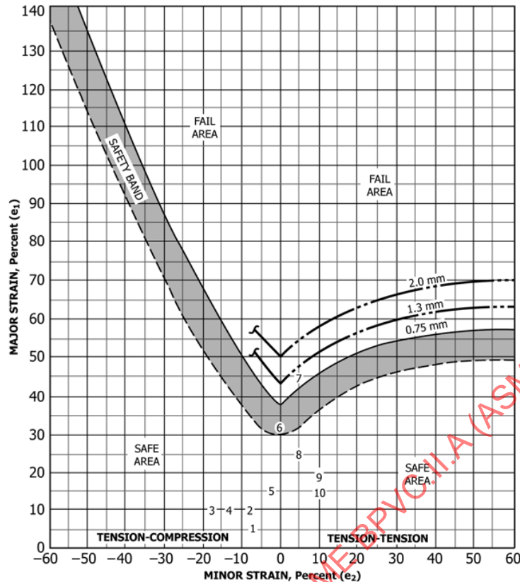
FIG. X4.1 Forming Limit Curve
