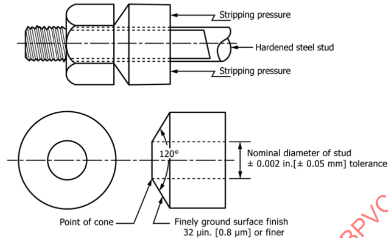
FIG. 2 Cone-Proof Test
