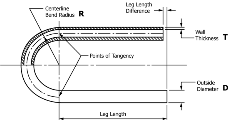
FIG. 1 Bent Portion of U-Tube
