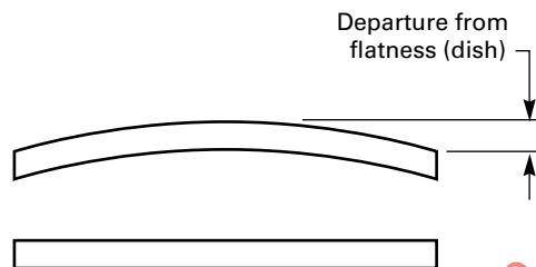
FIG. 10 BAND SAW FLATNESS (DISH) TOLERANCE
