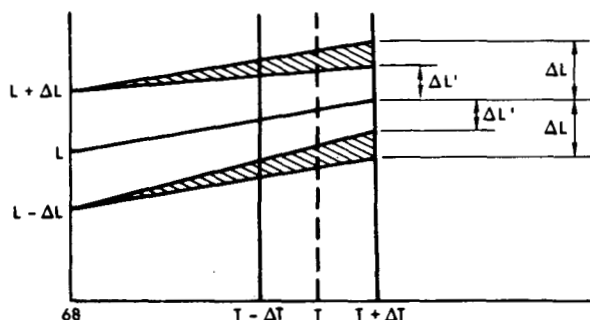
FIG. 6 Effect of uncertainties of coefficients of expansion on permissible tolerances. Part nominal size of L with tolerance \pm \Delta L . Tolerance is reduced to \pm \Delta L' when mean temperature is T \pm \Delta T .
