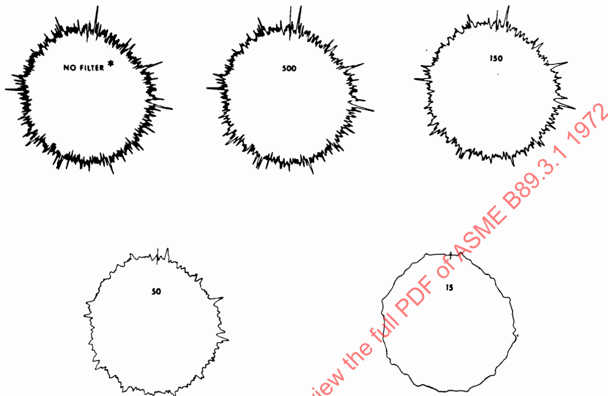
FIG. D1 POLAR PROFILES AT VARIOUS FILTER VALUES
