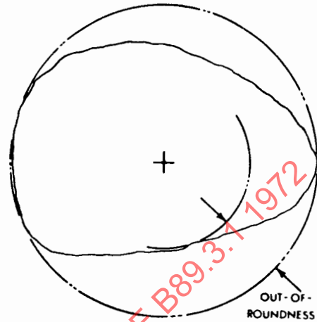
FIG. C5 MINIMUM CIRCUMSCRIBED CIRCLE
