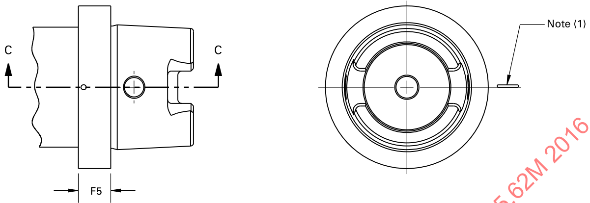
Figure 1-2-2 HSK Form C
