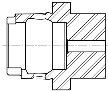
(c) Form C
