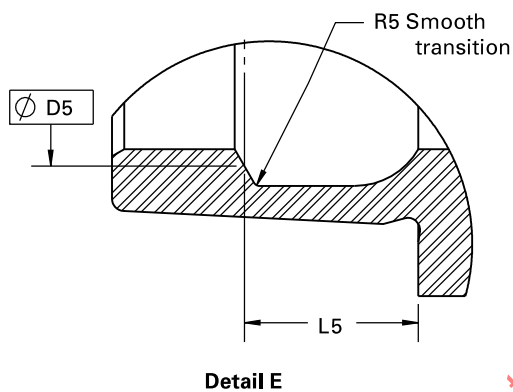
NOTES: Table 1-4-1 for dimension values. The texture is per ASME B46.1. Unless otherwise specified, surface texture, R_a , is 3.2 \mu\text{m} . All sharp edges.
