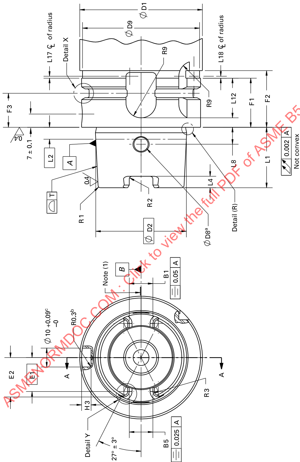
Figure 1-6-1 HSK Form T
