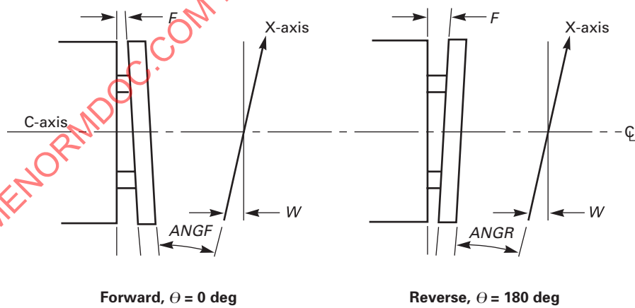
Fig. 7.8.2.1-2 Schematic Showing the Angles Involved When Measuring Cross-Slide Squareness to the Spindle Axis
