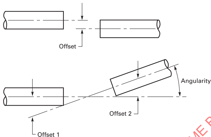
Fig. 8.2-1 Illustration of Angularity and Offset Between Two Axes of Rotation
