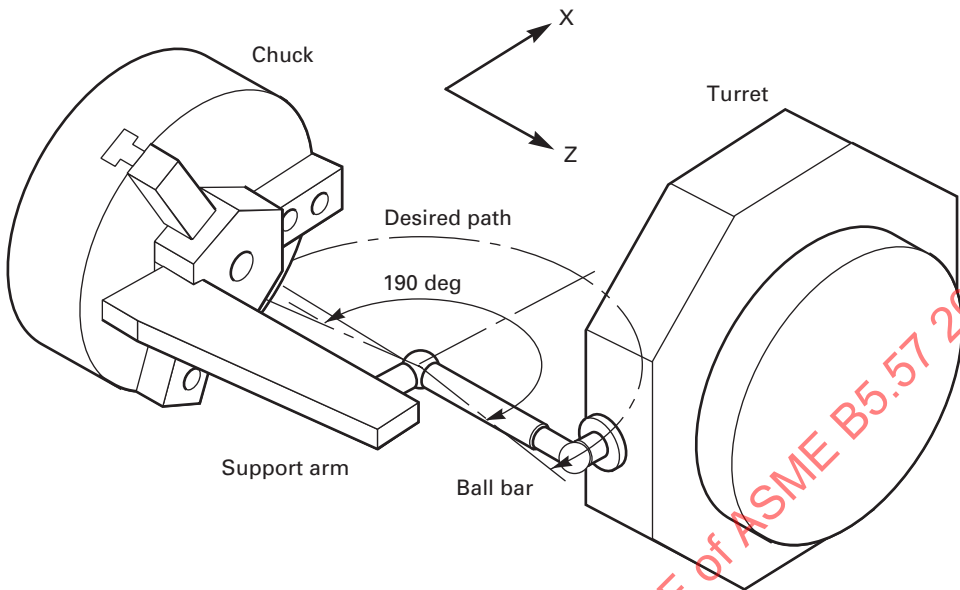
Fig. 7.9.3-1 Typical Ball Bar Setup for the 190-deg Test on a Lathe
