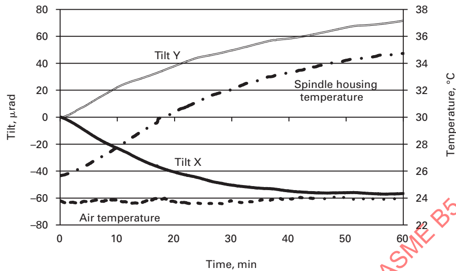
Fig. 7.7.2.1-2 Tilts of the Axis Average Line, Spindle Warm-Up Test
