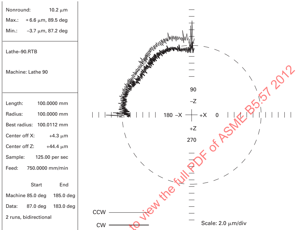
Fig. 7.9.4-2 Typical Results of a 100-deg Ball Bar Test
