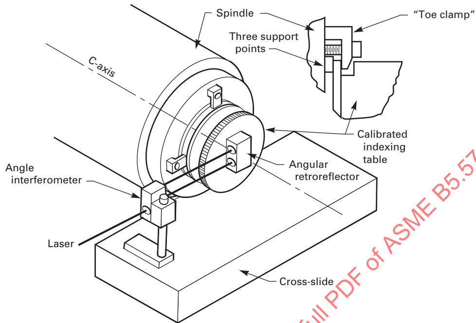
Fig. 7.5.2-1 Schematic for the Measurement of Angular Positioning Using an Indexing Table and a Laser Interferometer
