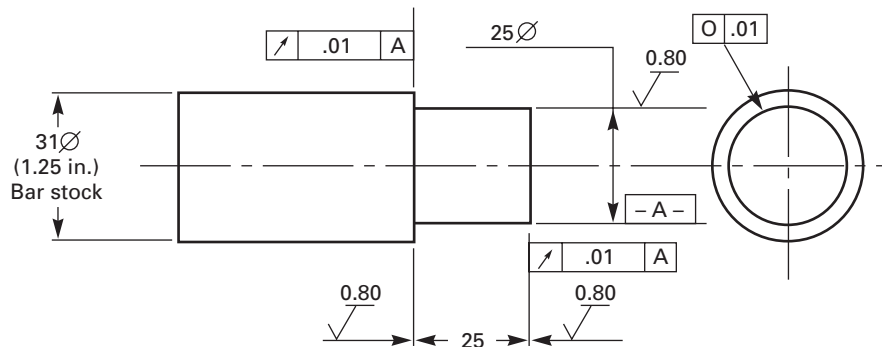
Fig. 8.4.2-1 Test Part for Determining the Location of a Tool-Setting System and Tool-Setting-System Drift
