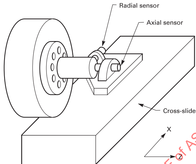
Fig. 6.2.1.4-1 Setup Showing Two Displacement Sensors Used to Measure the Environmental Temperature Variation Error (ETVE) Between a Nominal Tool Location and a Work Spindle
