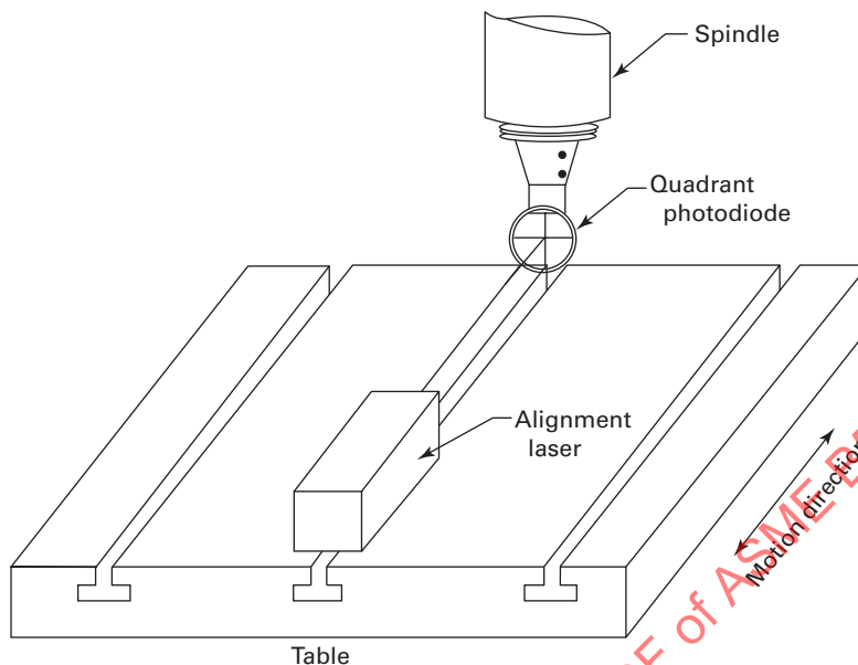
Fig. 7.3.1.3-1 Test Setup for Measuring Straightness Using an Alignment Laser
