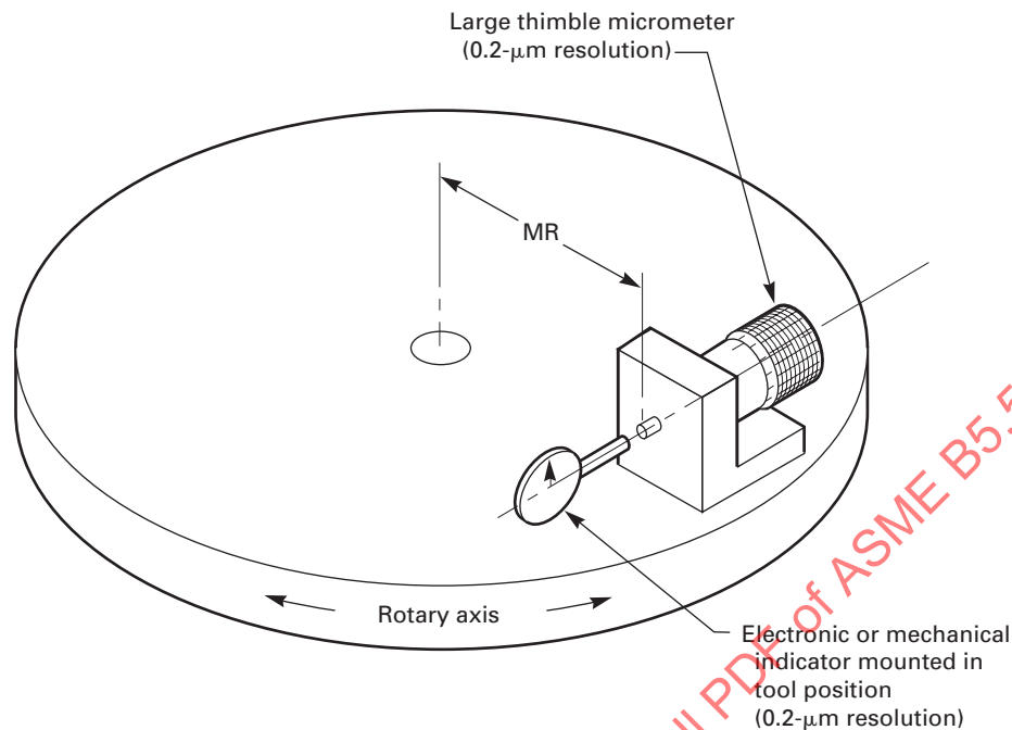
Fig. 7.5.8.2-1 Typical Setup for Periodic Angular Error Measurement Using Mechanical Means
