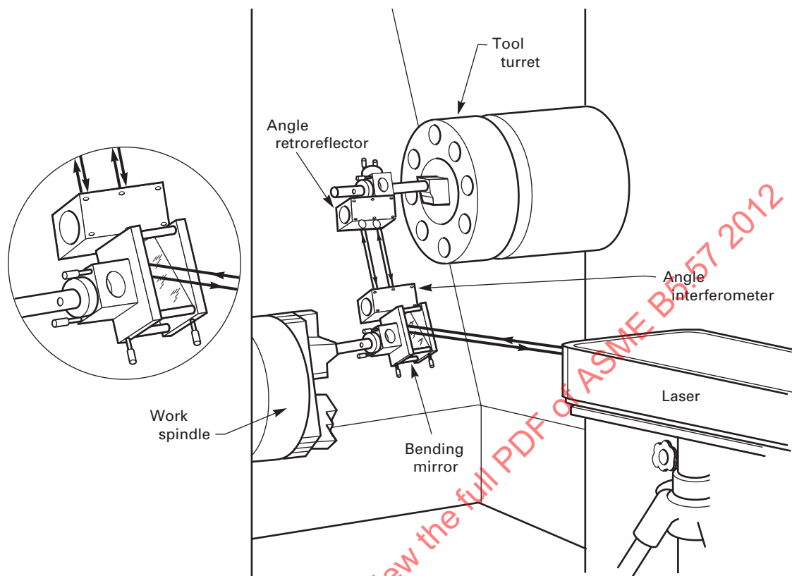
Fig. 7.4.1-1 Typical Setup for Measuring the Angular Error Motion (Yaw) of the Cross-Slide on a Group 1 Machine
