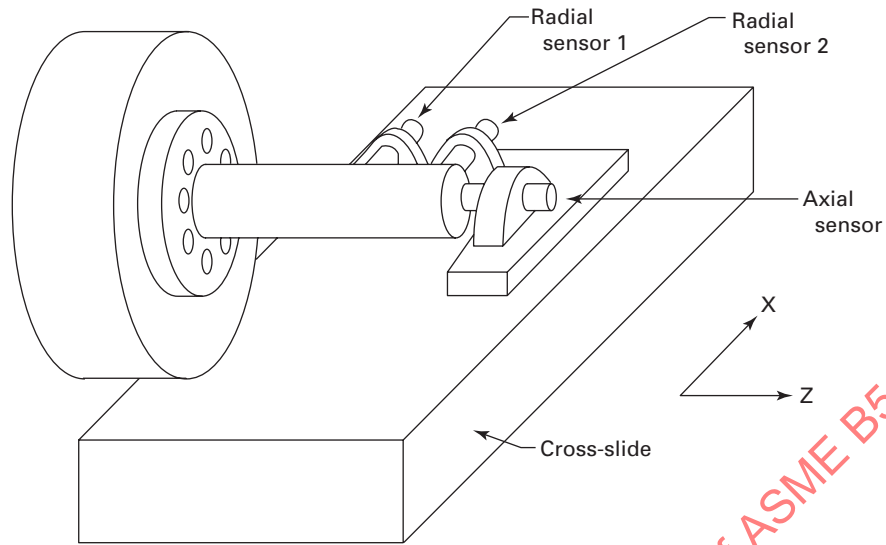
Fig. 7.6.3-1 Test Setups for Measuring Spindle Error Motions in the Case of Fixed Sensitive Direction
