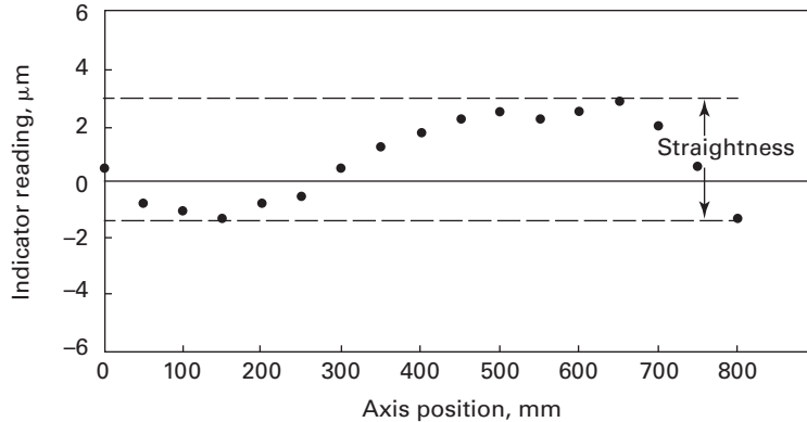
Fig. 7.3.2-1 Typical Plot Showing Straightness Data With the Straightness for a Particular Axis Clearly Labeled
