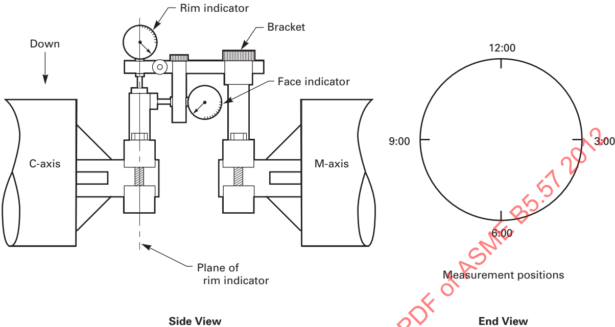
Fig. 8.2.1-1 Typical Setup for the Rim-and-Face Test
