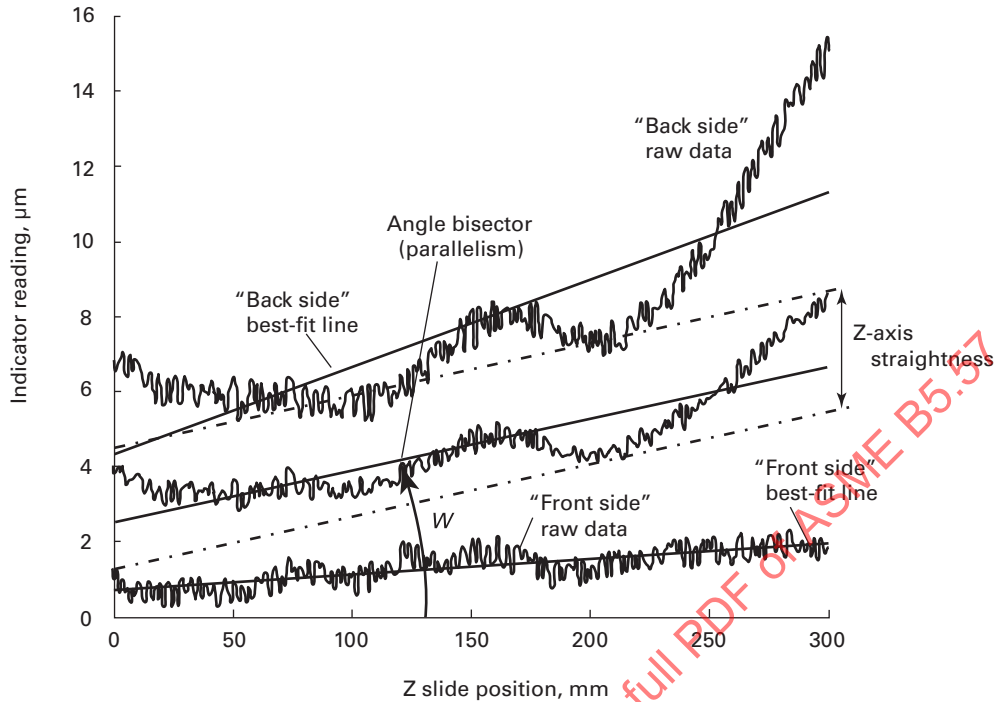
Fig. 7.8.3.2-2 Typical Data From a Parallelism Measurement Using the Turned Cylinder Method
