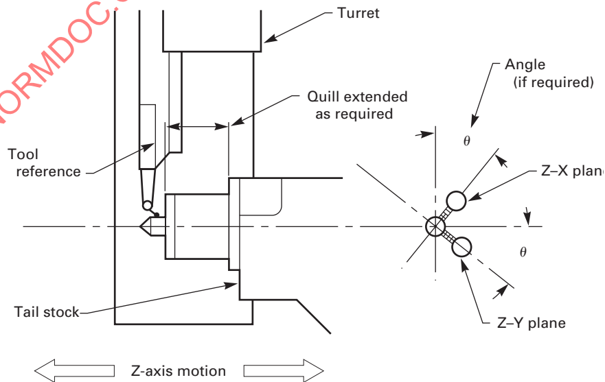
Fig. 8.2.5-1 Schematic of the Measurement of Parallelism of the Z-Axis to the Axis of a Movable Tail Stock
