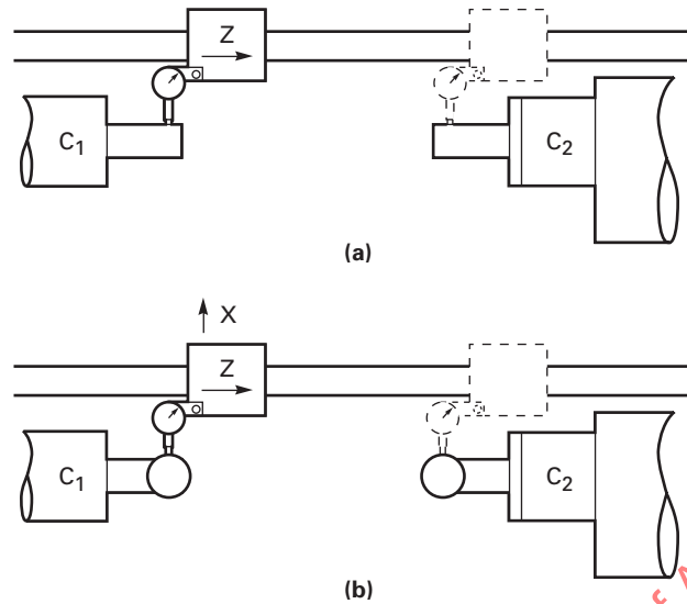
Fig. 8.2.5.1-1 Setup for Measuring Tail Stock Alignment Using the In-Feed (Z) Axis
