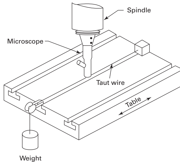
Fig. 7.3.1.2-1 Test Setup for Measuring Straightness Using a Taut Wire
