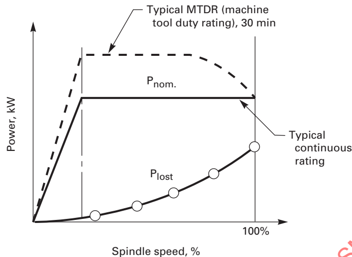
Fig. 7.10.2-1 A Typical Plot of the Power Loss in the Spindle Idle Run Loss Test
