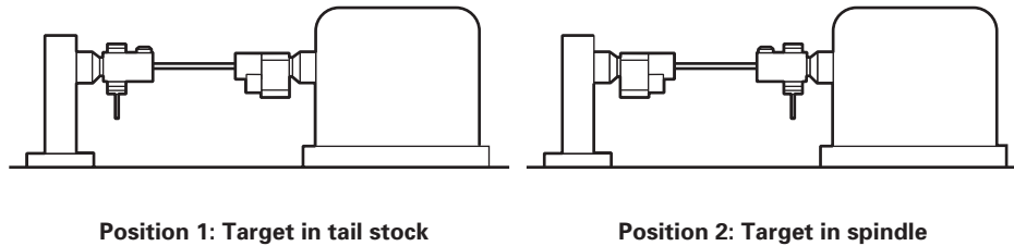
Fig. 8.2.3-1 Rotation Axes Alignment Using an Optical Alignment Laser
