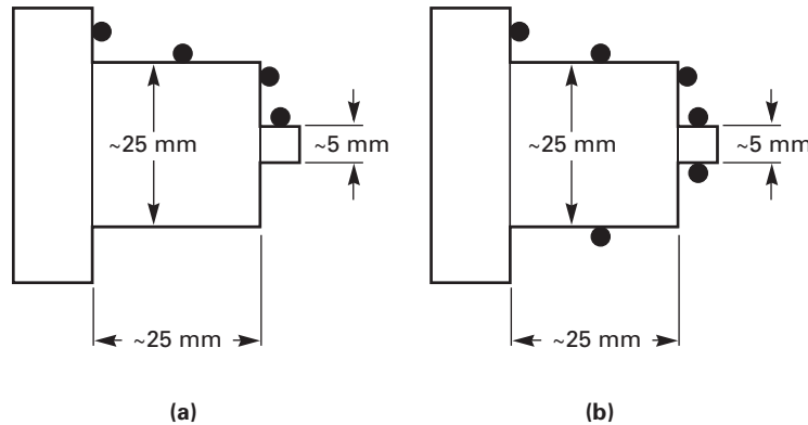
Fig. 8.6.2-1 Approximate Location of Probed Points, Depending on Probe Configuration, When Measuring a Machined Test Part
