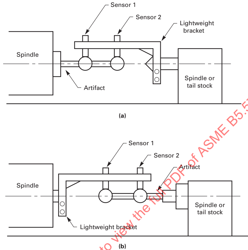
Fig. 8.2.4-1 Two-Sphere Setup for the Alignment of Two Rotation Axes
