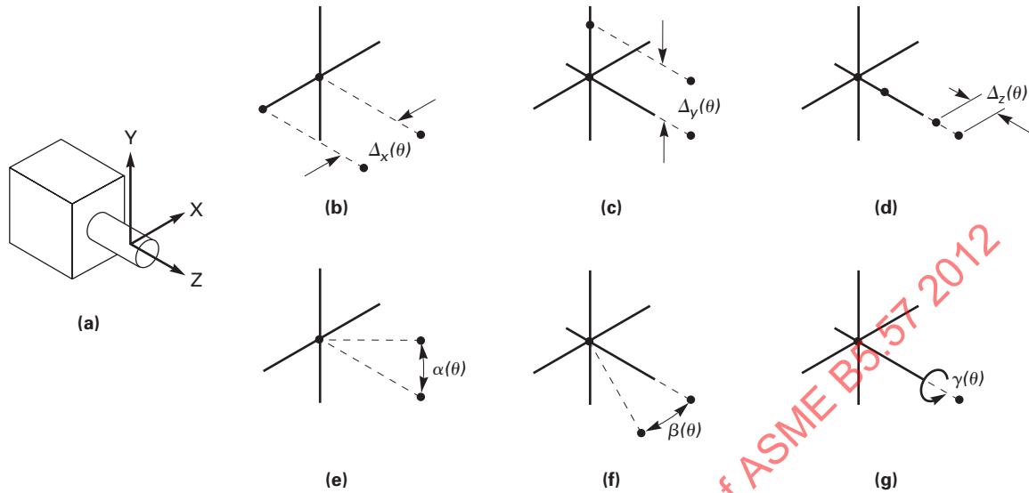
Fig. 4-1 The Six Basic Error Motions of an Axis of Rotation
