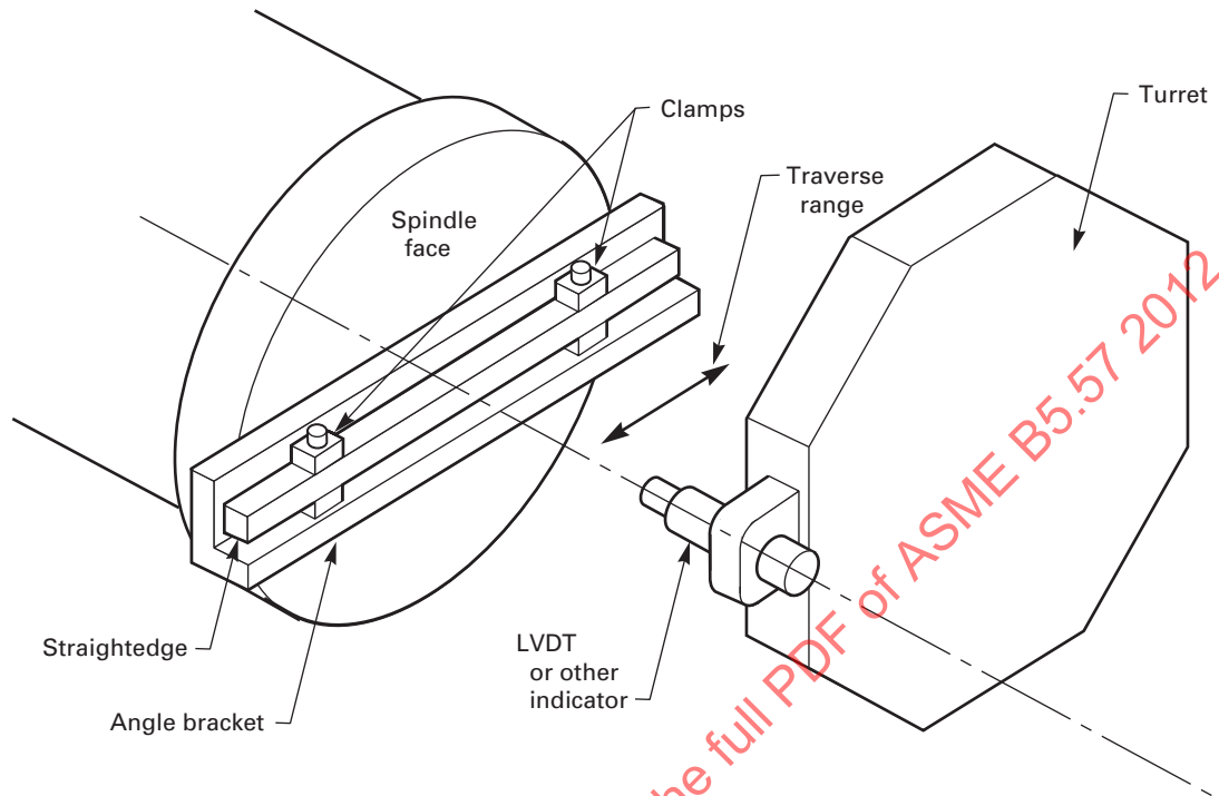
Fig. 7.8.2.1-1 Setup for Measuring Squareness of the Cross-Slide to the Work Spindle Using a Mechanical Straightedge
