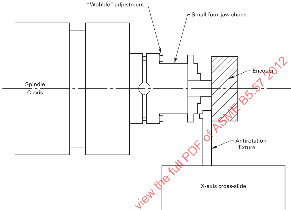
Fig. 7.5.5-1 Typical Setup for Measuring the Angular Positioning Accuracy of a Rotary Axis Using an Angular Encoder
