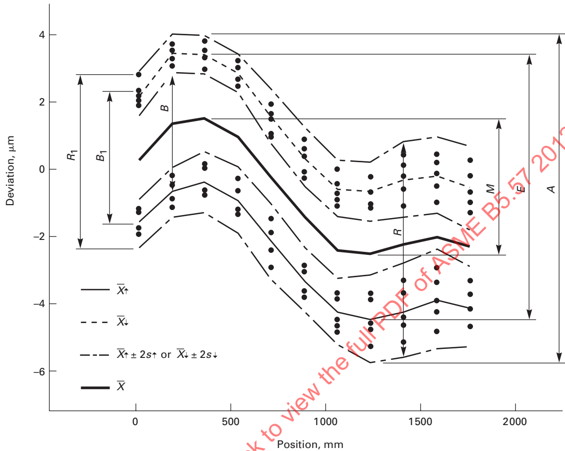
Fig. 7.2.7-1 The Full Data Set for the Positioning Deviations of an Axis
