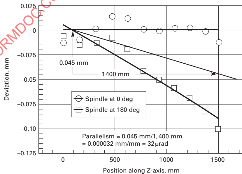
Fig. 7.8.4-2 Graphing of Both Straightness Measurements for Twice the Angle of Parallelism
