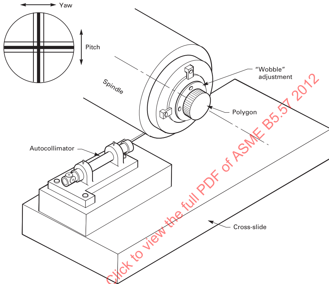
Fig. 7.5.4-1 A Polygon Mounted to a Spindle Axis
