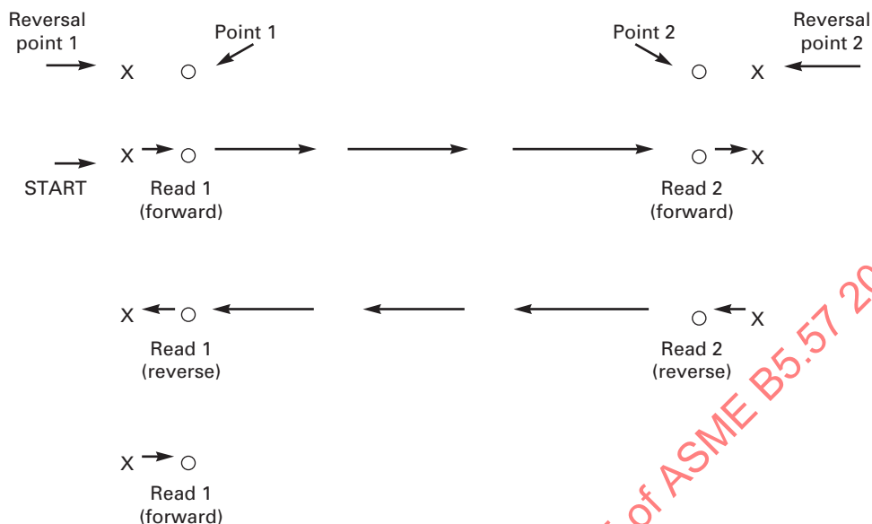
Fig. 7.7.3.1-1 Path for Measuring Thermal Distortion Caused by Moving Linear Axes
