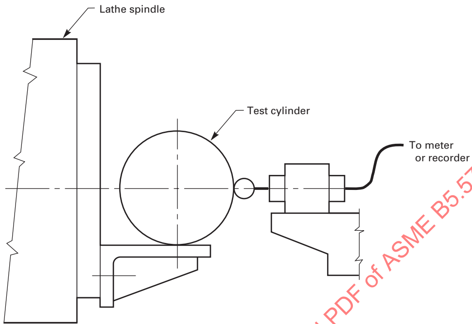
Fig. 7.8.2.3-1 Cylinder Reversal for Cross-Slide Squareness
