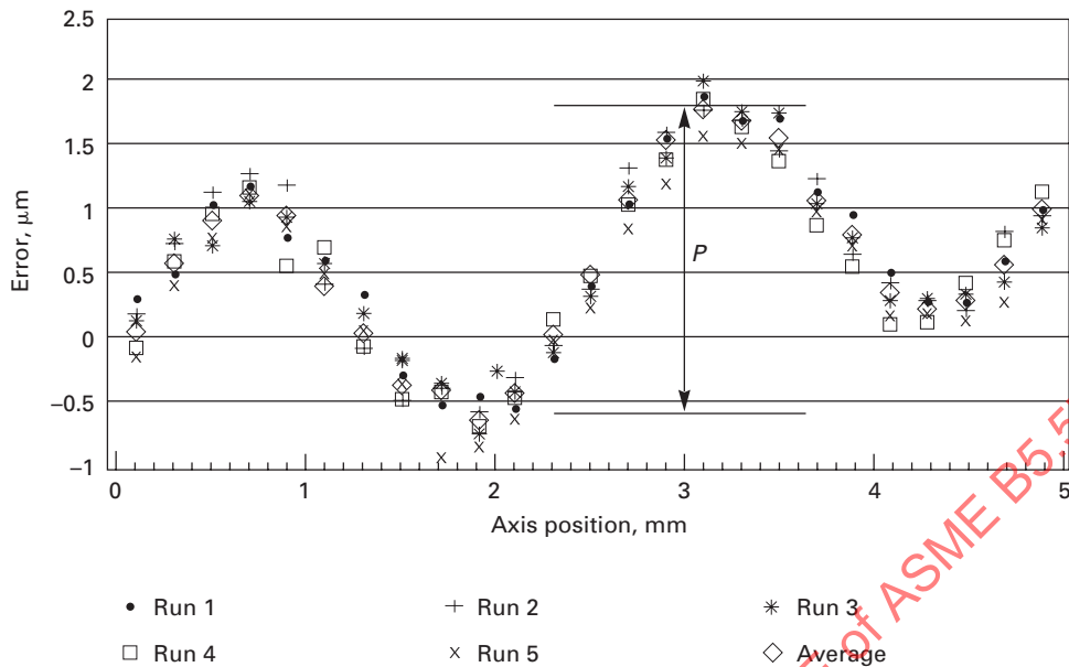
Fig. 7.2.8-1 Periodic Error of a Linear Axis (Unidirectional)
