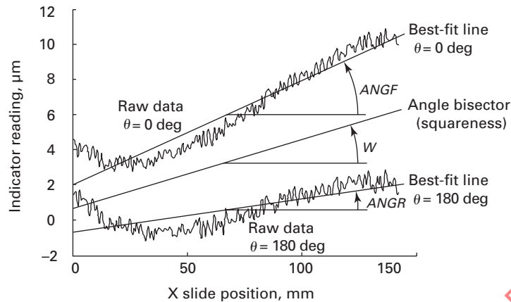
Fig. 7.8.2.1-3 Typical Data From a Cross-Slide Out-of-Squareness Measurement
