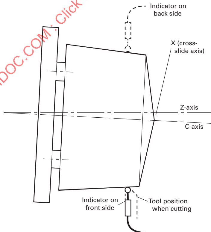
Fig. 7.8.3.2-1 Z-Slide Parallelism Schematic Showing the Test Cylinder
