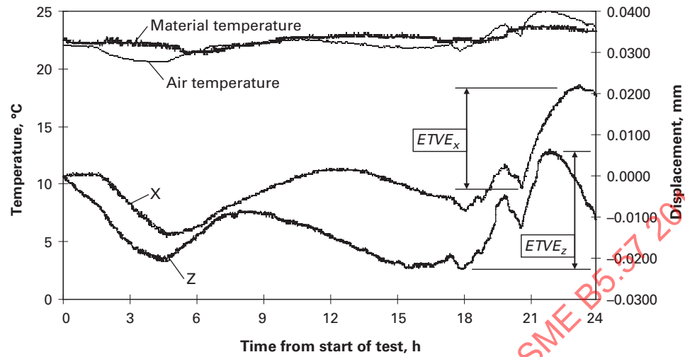
Fig. 6.2.1.4-3 Graph of Environmental Temperature Variation Error (ETVE) Data
