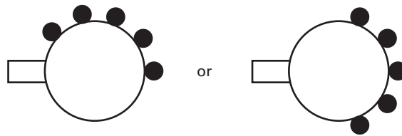
Fig. 8.6.3-1 Approximate Location of Probed Points, Depending on Probe Configuration, When Measuring a Test Sphere
