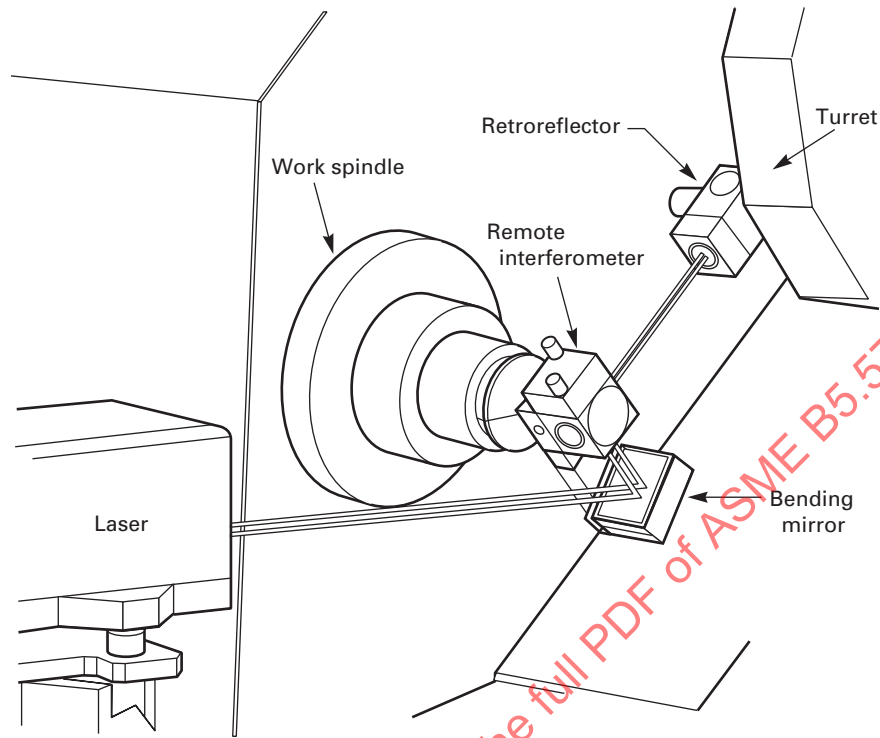
Fig. 7.2.3-1 Typical Setup for a Laser Interferometer
