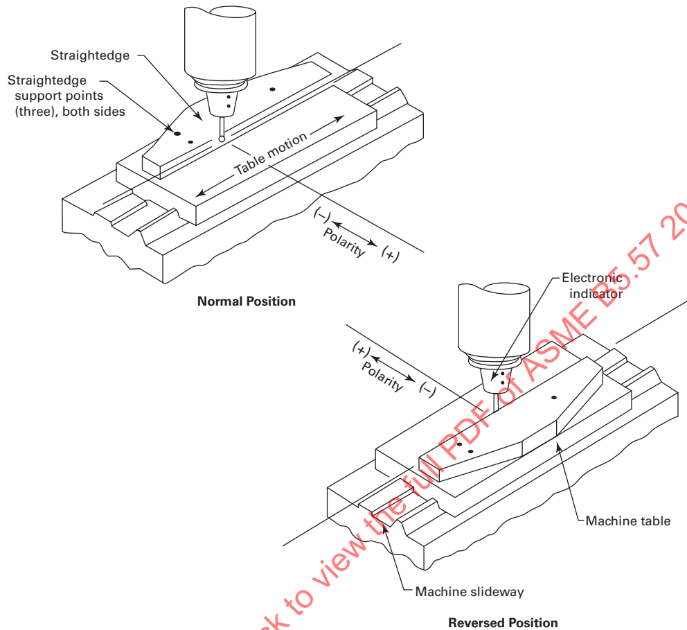
Fig. 7.3.1.1-1 Setup for Measuring Straightness Using an Electronic Indicator and a Mechanical Straightedge
