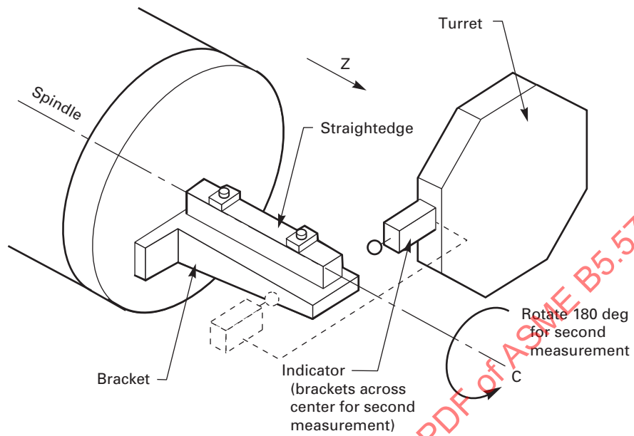
Fig. 7.8.3.1-2 Setup for Straightedge Rotation on a Horizontal Spindle Lathe for Measuring Z-Axis Parallelism to the C-Axis
