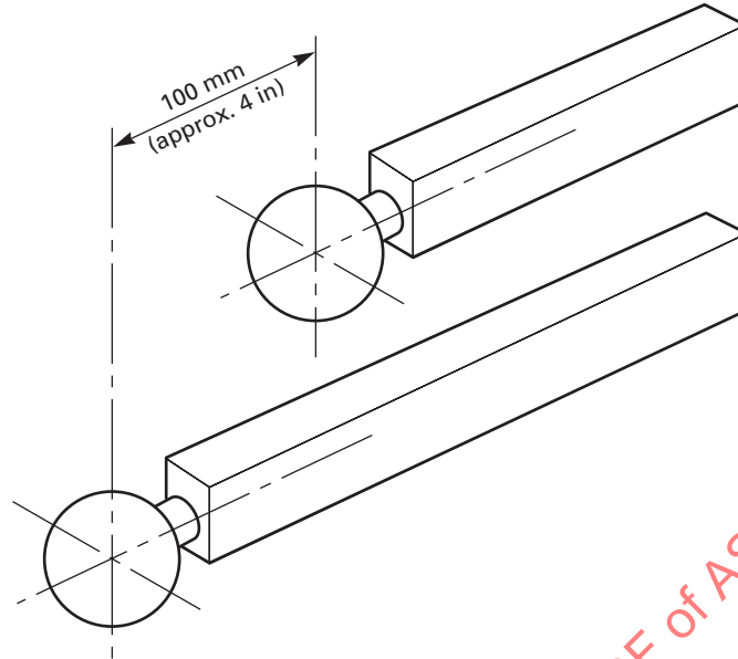
Fig. 8.3.2-1 Example Tool Holders to Be Used for Turret Repeatability
