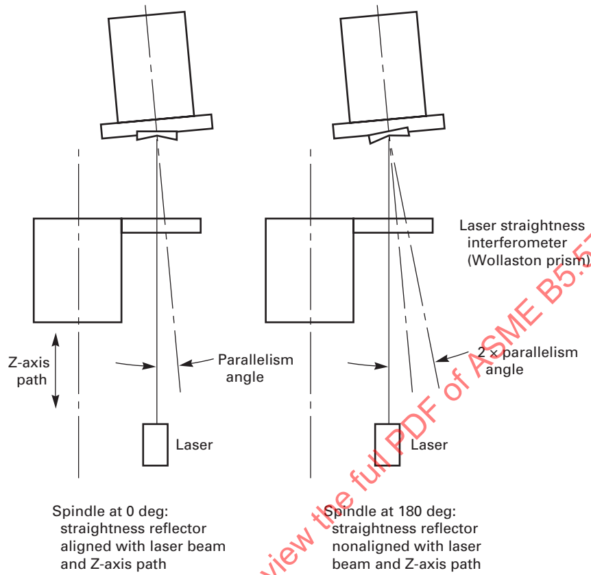
Fig. 7.8.4-1 Dual Straightness Measurement for Parallelism
